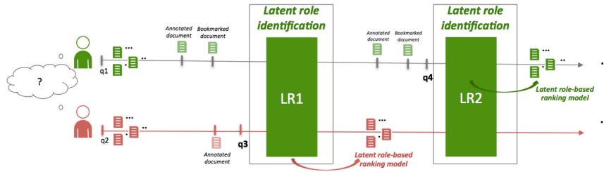
Figure 1: Unsupervised latent role learning methodology.
