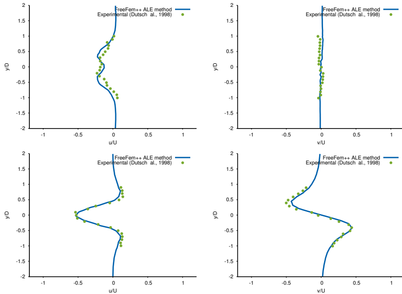
Figure 2: Comparison of the computed and referenced solutions along the line x = -0.6 * D (top) and x = 1.2 * D (bottom) for the values of \mathbf{u} = (u, v) at t = \frac{59}{12}T .
