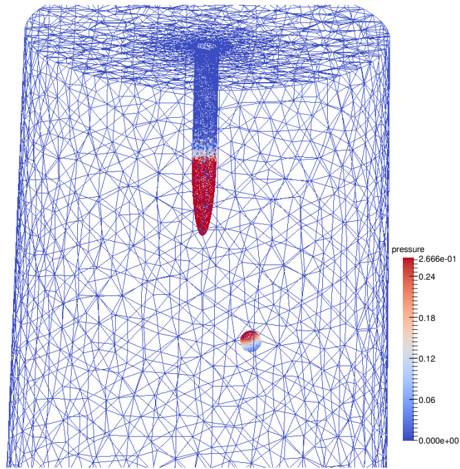
Figure 5: The predicted pressure contours on the needle and cell surface as the needle moves toward the cell with \alpha_f = 0.7 , Da = 0.321 , and Re = 0.103 .
