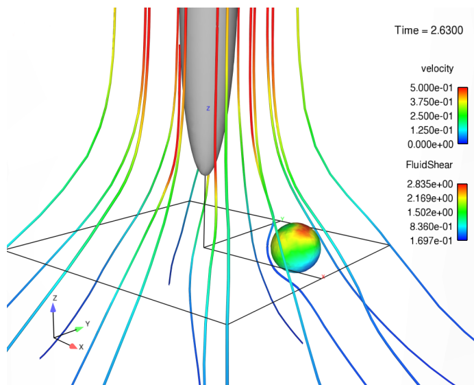
Figure 6: The predicted streamlines and shear stress on the cell surface as the needle moves toward the cell with \alpha_f = 0.7 , Da = 0.321 , and Re = 0.103 .
