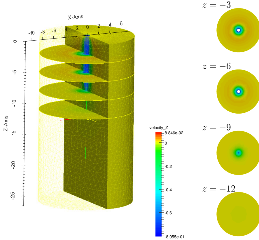
Figure 3: The predicted contours of velocity along the z-direction resulting from the needle (blue) motion in interstitial fluid with \alpha_f = 0.7 , Da = 0.321 , and Re = 0.103
