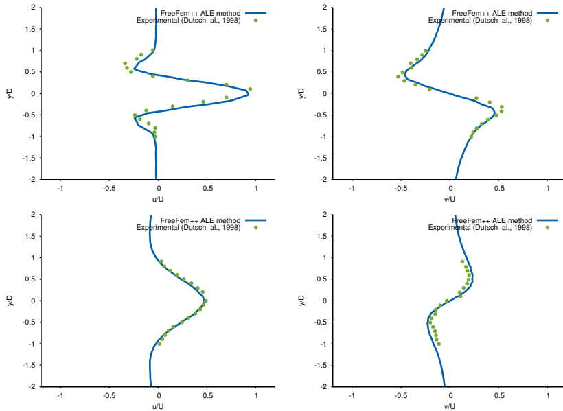
Figure 1: Comparison of the computed and referenced solutions along the line x = -0.6 * D (top) and x = 1.2 * D (bottom) for the values of \mathbf{u} = (u, v) at t = \frac{55}{12}T .
