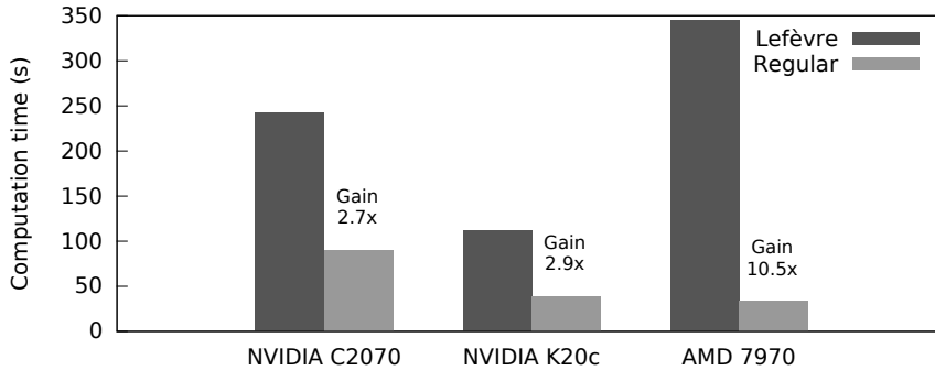
FIG. 5.1. HR-case searches computation times over I_{0..1023} on various GPUs, using OpenCL from CUDA 7.5 (352.68 driver) and from the AMD SDK 2.9.1 (Catalyst Omega 14.12 driver). The performance gains on top of the bars correspond to the Lefèvre over regular ratios.
