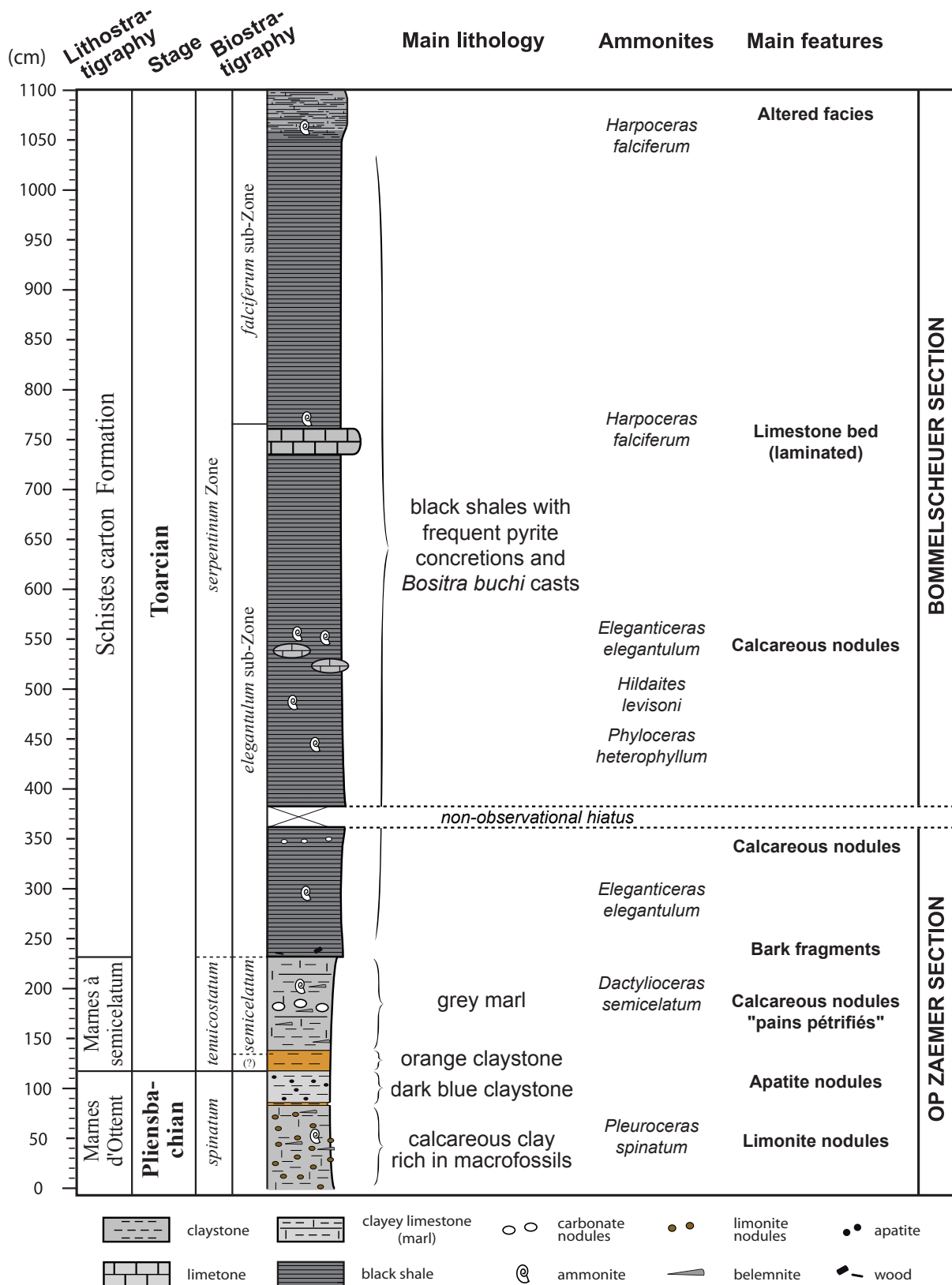
Figure 2. Lithostratigraphy, biostratigraphy and main lithological description of the composite section of Bascharge spanning the Late Pliensbachian to Early Toarcian intervals of the Op Zämer and Bommelscheuer outcrops.
