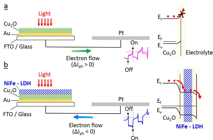
Figure 4. Schematics of photogenerated electron transfer occurring in a PEC system using (a) bare \text{Cu}_2\text{O} and (b) modified \text{Cu}_2\text{O}/\text{NiFe-LDH} (20s) electrodes. The reversal of the electron flow at low voltages is indicated as well as the corresponding band diagrams (red dots denote electrons).
