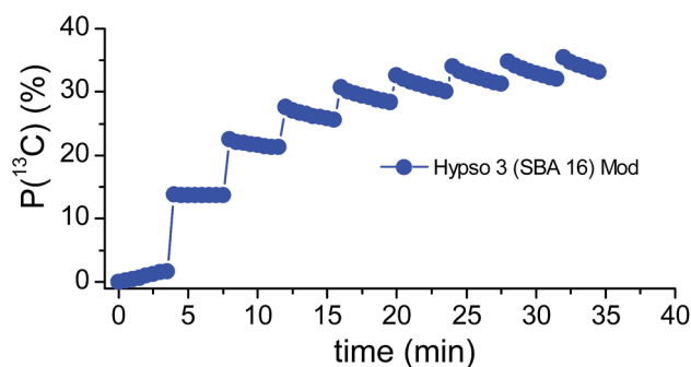
Fig. 4 Left ^1\text{H} \rightarrow ^{13}\text{C} CP-DNP performed on HYPISO-3 material (67 \mu\text{mol}_{\text{NO}} \text{cm}^{-3} ) impregnated with a 3 M solution of [1\text{-}^{13}\text{C}] -acetate in D 2 O. P(^{13}\text{C}) 36% is reached in 32.5 min with ^1\text{H} \rightarrow ^{13}\text{C} CP applied at 4 min intervals.
