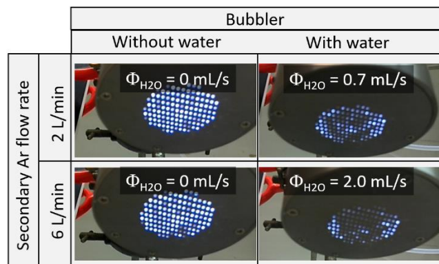
Figure 2. Influence of the water vapor and secondary Ar flow rates on the apparent post-discharge stability, for P=80 W, Φ(Ar) = 30 L.min -1 .
