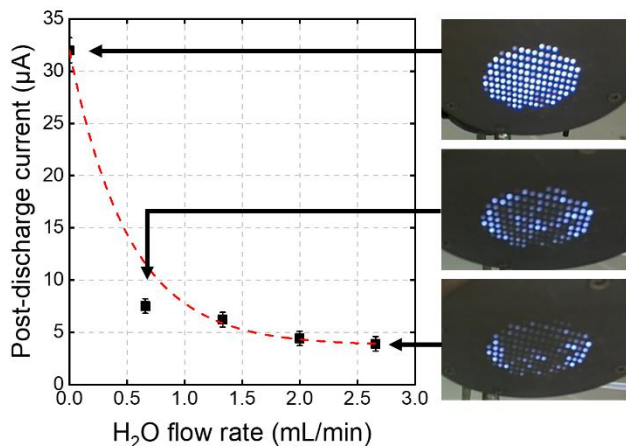
Figure 3. Influence of the H 2 O flow rate on the post-discharge current. Gap = 10 mm. Ar flow rate = 30 L.min -1 , RF power = 80 W.
