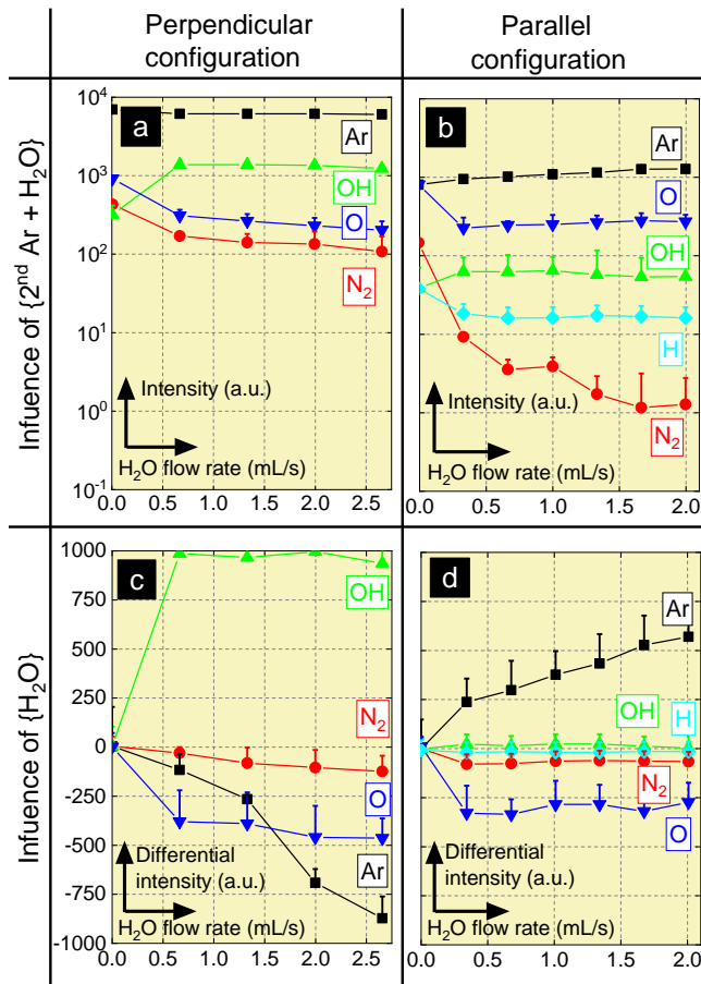
Figure 4. OES measurements showing the effect of the \text{H}_2\text{O} flow rate on the emission and differential emission of OH, O, \text{N}_2 , Ar and H species (Ar flow rate = 30 \text{ L min}^{-1} , power = 80 \text{ W} ). The differential emission is given by \varepsilon_{\text{diff}}\{\text{H}_2\text{O}\} = \varepsilon\{2^{\text{nd}} \text{ Ar} + \text{H}_2\text{O}\} - \varepsilon\{2^{\text{nd}} \text{ Ar}\}
