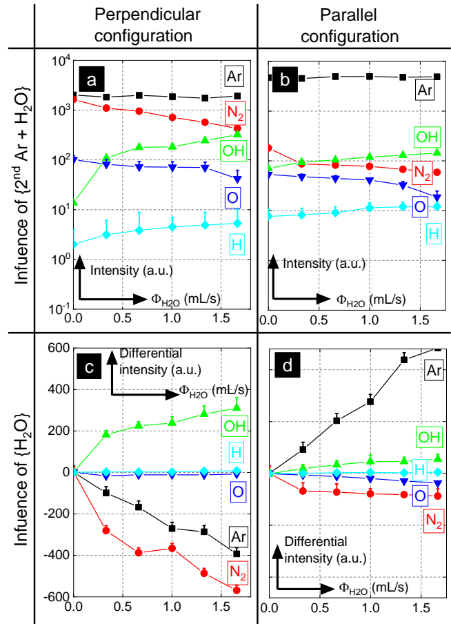
Figure 5. Mass spectrometry measurements showing the effect of the \text{H}_2\text{O} flow rate on the intensity and differential intensity of OH, O, \text{N}_2 , Ar and H species (Ar flow rate = 30 \text{ L min}^{-1} , power = 80 \text{ W} ).
