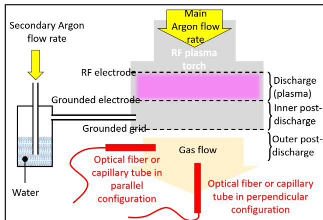
Figure 1. Schematic diagram of the experimental setup and location of the three discharge regions.
