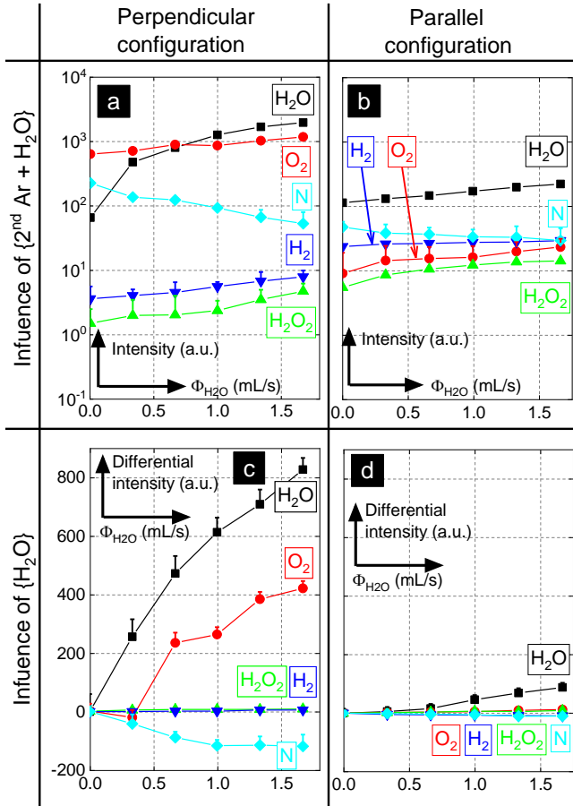
Figure 6. Mass spectrometry measurements showing the effect of the H 2 O flow rate on the intensity and differential intensity of H 2 O, O 2 , H 2 O 2 , H 2 and N (Ar flow rate of 30 L min -1 and RF power of 80 W).
