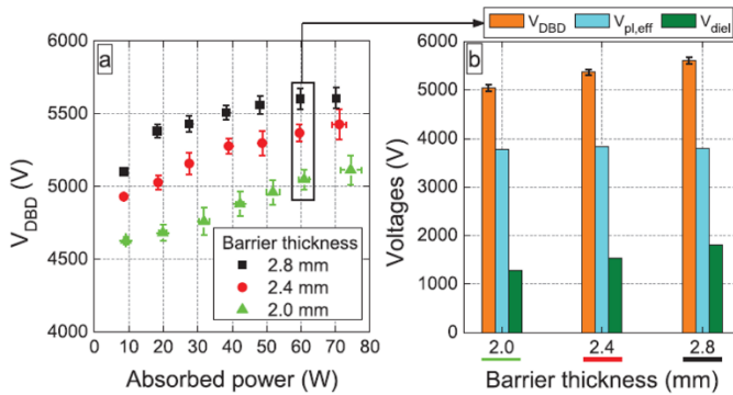
Figure 3. (a) Applied voltage ( V_{DBD} ) as a function of absorbed power for three different dielectric thicknesses, and (b) voltage components as a function of the dielectric thickness at a given absorbed power P_{obs} = 60 W; f = 28.6 kHz; \Phi(CO_2) = 200 mL n ·min -1 .
