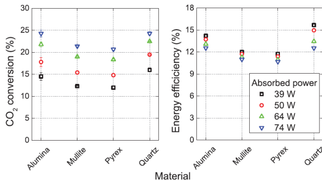
Figure 5. (a) CO 2 conversion and (b) energy efficiency for different values of the absorbed power and for four different dielectric materials; f = 27.1 kHz; \Phi(\text{CO}_2) = 200 mL n ·min -1 .
