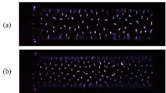
Figure 4. Pictures of the microdischarges observed through the pyrex and the outer mesh electrode, at the same power, frequency and flow rate (for a camera aperture of 1/100 s). The barrier thickness is (a) 2.0 mm, (b) 2.8 mm.
