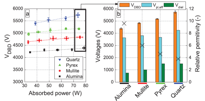
Figure 6. (a) RMS applied voltage ( V_{\text{DBD}} ) as a function of absorbed power for four different dielectric materials at f = 27 kHz, and (b) RMS voltage components as a function of the dielectric material at a given absorbed power P_{\text{obs}} = 75 W; \Phi(\text{CO}_2) = 200 mL n ·min -1 . The relative permittivities of the materials are indicated with crosses, referring to the right y-axis.
