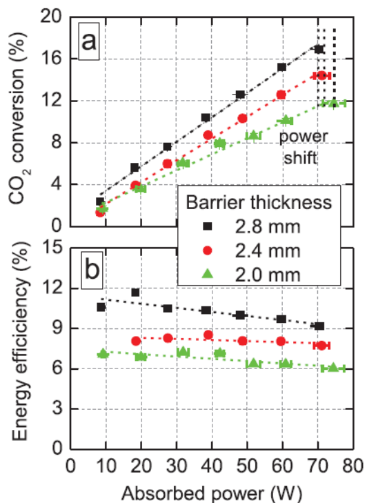
Figure 2. (a) CO 2 conversion and (b) energy efficiency as a function of the absorbed (plasma) power for three different dielectric thicknesses (2.0, 2.4 and 2.8 mm); f = 28.6 \text{ kHz} ; \Phi(\text{CO}_2) = 200 \text{ mL.n}^{-1} .
