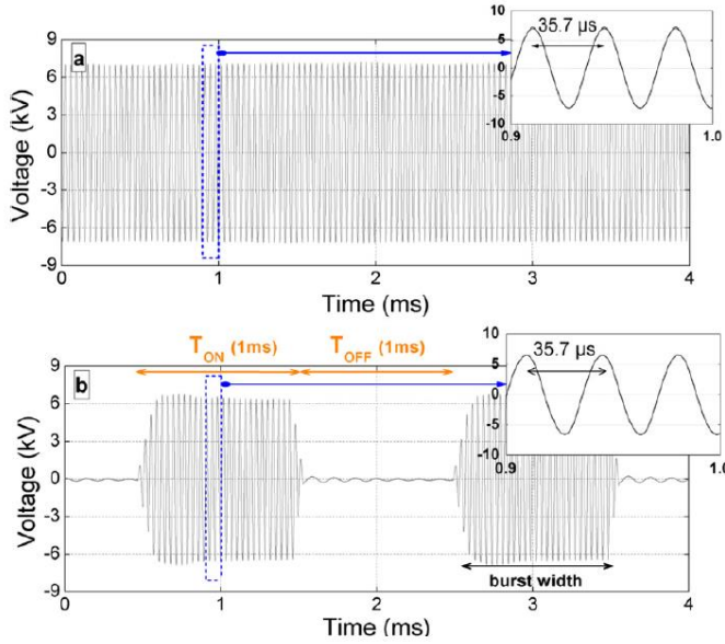
Figure 2. High voltage signals applied to the discharge, with frequency of 28.6 kHz (or period of 35.7 μs), in (a) pure AC mode, and (b) burst mode, with a duty cycle of 50% ( T_{ON} = T_{OFF} = 1 ms).
