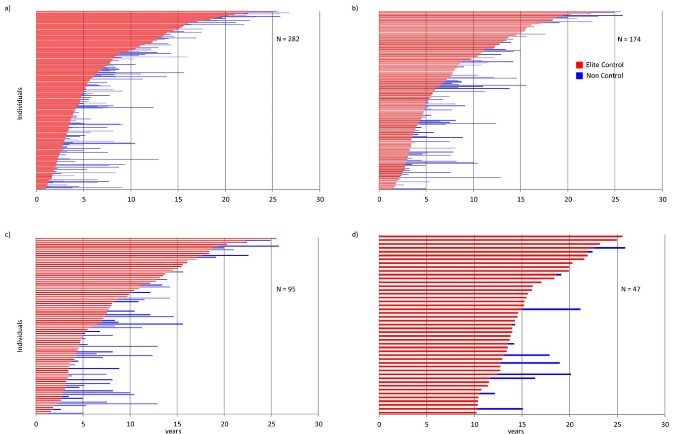
Figure 1. Total ART-naïve follow-up time spent as an elite controller for 4 of the best performing definitions: a) A F , b) E F , c) F F , and d) J F using the CASCADE dataset. A: HIV-positive \geq 6 months, with \geq 2 consecutive HIV-RNA < 75 copies/ml; E: HIV-positive \geq 1 year, with \geq 3 consecutive HIV-RNA < 75 copies/ml spanning \geq 12 months F: HIV-positive \geq 1 year, with \geq 3 consecutive HIV-RNA < 75 copies/ml spanning \geq 12 months with no previous blips \geq 1000 copies/ml, J: HIV-positive \geq 10 years, with \geq 90\% of HIV-RNA ( \geq 2 HIV-RNA ever) < 400 copies/ml. doi:10.1371/journal.pone.0086719.g001
