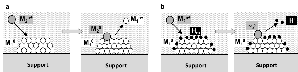
Figure 8. Schematic illustration of the surface redox methods: (a) Direct reduction of \text{M}_2^{n+} ions by \text{M}_1^0 metal particle, also called galvanic replacement reaction; (b) Reduction of \text{M}_2^{n+} ion by active H adsorbed on \text{M}_1^0 metal particle resulting from \text{H}_2 dissociation or activation of a reducing agent on \text{M}_1^0 .
