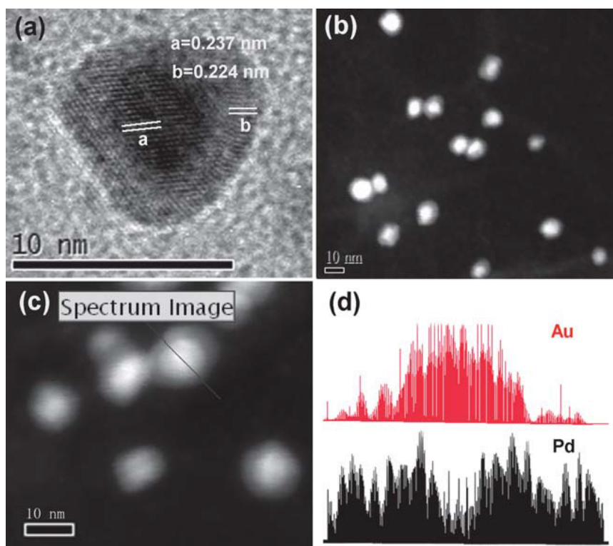
Figure 5. HRTEM image (a) of a single Au core-Pd shell nanoparticle dispersed on graphene. STEM-HAADF image (b) of the hybrids. EELS (electron energy loss spectroscopy) spectrum images (c,d) of a single nanoparticle—Adapted with permission from [77]. Copyright 2011, Royal Society of Chemistry.
