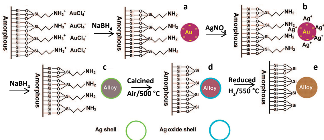
Figure 2. Schematic illustration of the procedure of synthesis of SiO_2 -supported Au-Ag alloy nanoparticles. (a) Initially formed Au particles; (b) AgNO_3 adsorbed on the Au particles; (c) Au-Ag nanostructure with alloy core surrounded by a silver shell; (d) Au-Ag nanostructure with more gold-rich alloy core covered by a Ag oxide shell; (e) random alloy of Au-Ag nanoparticles on SiO_2 support—Adapted with permission from [42]. Copyright 2009, American Chemical Society.
