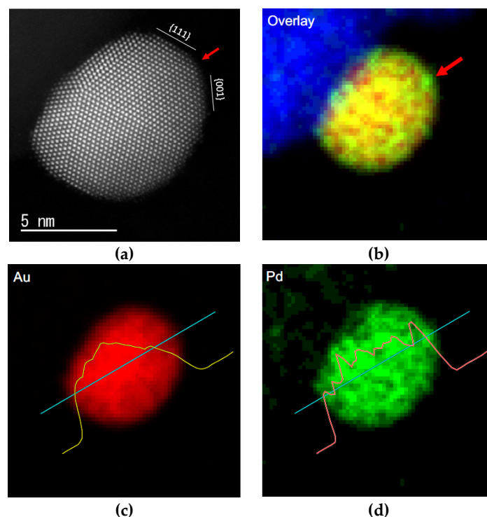
Figure 1. A Au-Pd nanoparticle on \text{TiO}_2 support (Co-DP with NaOH at pH 6.5); (a) High-resolution STEM (scanning transmission electron microscopy) image; (b,c,d) high resolution EDS analysis of the same particle—Adapted with permission from [30]. Copyright 2014, Springer.
