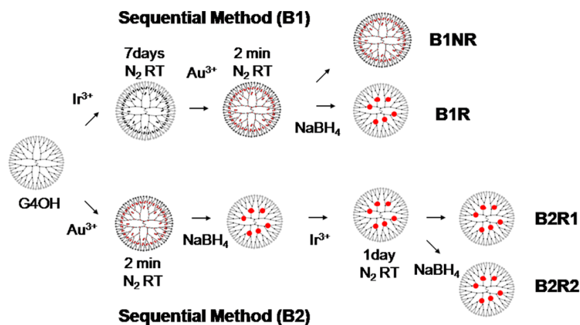
Figure 7. Four sequential method of preparation of bimetallic Au-Ir particles in dendrimers before impregnation on alumina: (B1) \text{IrCl}_3 then \text{HAuCl}_4 adsorption (B1NR) and reduction with \text{NaBH}_4 (B1R); (B2) \text{HAuCl}_4 adsorption and reduction with \text{NaBH}_4 then \text{IrCl}_3 adsorption (B2R1) and reduction with \text{NaBH}_4 (B2R2). Copied with permission from [90]. Copyright 2013, American Chemical Society.
