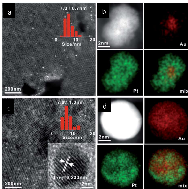
Figure 3. HAADF-STEM images and particle size distribution, typical EDS mappings of Au 50 Pt 50 /EP-TiO 2 after the photo-deposition (a,b) and after annealing at 350 °C (c,d). Adapted with permission from [48]. Copyright 2014, Royal Society Chemistry.
