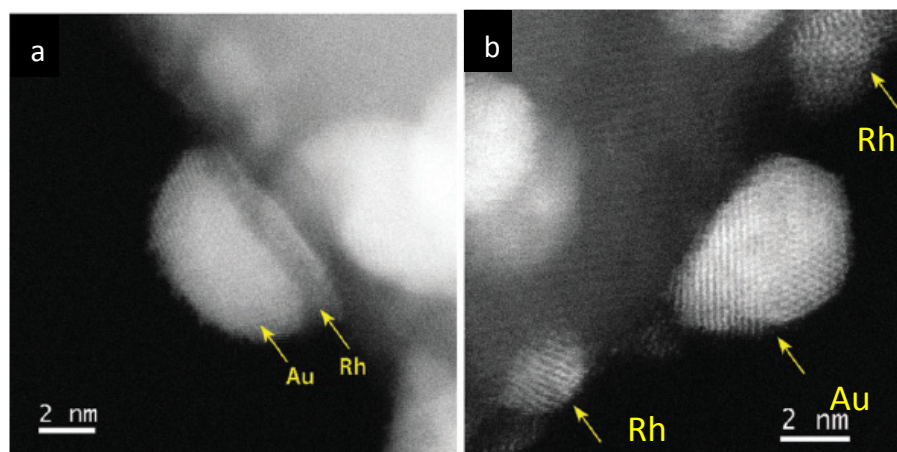
Figure 4. Representative aberration-corrected STEM-HAADF images of particles in Au-Rh/ \text{TiO}_2 sample: (a) a particle after treatment under \text{H}_2 at 350^\circ\text{C} showing a segregated “Janus-like” configuration with Au/Rh/ \text{TiO}_2 stacking; (b) particles after treatment under \text{O}_2 then \text{H}_2 at 350^\circ\text{C} showing metal segregation; smaller ones are Rh and larger ones are Au NPs (more contrasted)—Adapted with permission from [70]. Copyright 2015, Royal Society of Chemistry.
