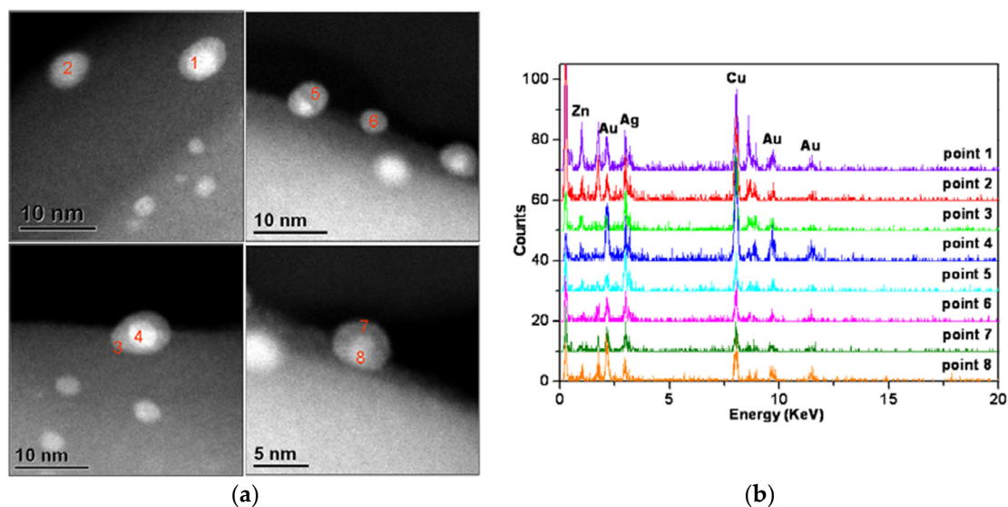
Figure 9. HAADF-STEM images (a) and the corresponding EDS spectra (b) for as-synthesized 2%Ag-2%Au/ZIF-8 sample. The copper signal originates from Cu grid—Adapted with permission from [127]. Copyright 2011, American Chemical Society.
