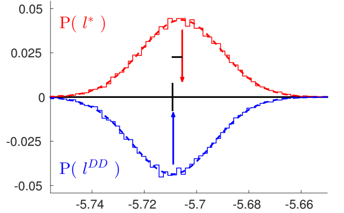
FIG. 6. (Colors online). Histogram of l_{\delta\mathbf{P}}^* (straight) and l_{\delta\mathbf{P}}^{\text{DD}} (reflected) obtained from the inference of S = 2 \cdot 10^4 empirical estimation of \delta\bar{\mathbf{P}} . See text for the details of the synthetic pairwise Ising model used for the simulations. Arrows indicate the corresponding histograms empirical means. The black vertical bar indicates the numerically exact value of \hat{l} , the exact model log-likelihood, whereas the black horizontal segment measures D/(2B) . Dotted lines represents the theoretical distributions, see eqs. (D4) and (D7). As predicted, see text, the average of l_{\delta\mathbf{P}}^{\text{DD}} coincides with \hat{l} , whereas the average of l_{\delta\mathbf{P}}^* suffers by a bias of D/(2B)
