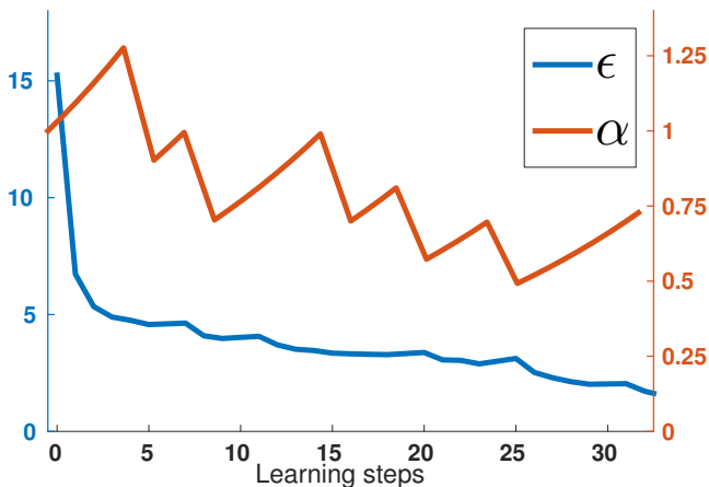
FIG. 2. (Colors online) Behavior of the pairwise Ising model inference of biological data through the Data-Driven algorithm. \varepsilon_t (lower blue curve, left axis) and of \alpha_t (upper red curve, right axis) during the algorithm running plotted against the iterative step number. Abscissa is not proportional to the running time as each step performs a different number M of MC sampling, see text. \alpha_t is raised (lowered) at every step where \varepsilon_t decreases (increases). The algorithm requires 100 \pm 5s to produce a set of fields \mathbf{X} satisfying the early-stop condition \varepsilon_t < 1 . Dataset as in fig. 1.
