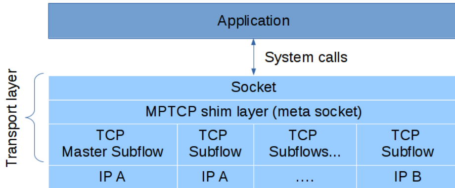
Figure 1: MPTCP: a shim layer in the stack. Subflows can share the IP address (using a different port) or have different IPs.
