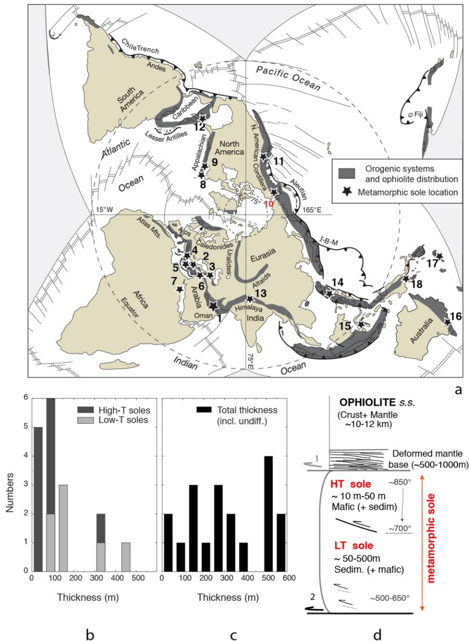
Figure 2 (a) Location of metamorphic soles and of the main large-scale obducted ophiolites worldwide (spanning late Proterozoic to Phanerozoic times); (b) and (c): histograms of thicknesses for metamorphic soles (after Table 1); (d) general structure of ophiolite soles (not to scale), emphasizing differences between the HT and LT sections. (temperature indications after Fig. 3a). Note the strongly deformed mantle section at the base of the ophiolite. Thrusts 1 and 2 as in figure 1b.
