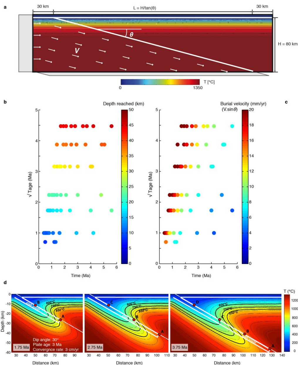
Figure S2. Thermo kinematic modelling of the temperature field associated with slab penetration into the mantle during subduction infancy; (a) Set-up of the numerical model. The initial temperature field is flat and depends on the thermal age of the oceanic lithosphere ( T_{age} ). V corresponds to the convergence velocity; (b) and (c): Variations, as a function of time and initial oceanic T_{age} , of the depth (left panel) and burial velocity ( V \cdot \sin \theta ; right panel) required for the tip of the slab to reach the temperature of 700°C. Depths of metamorphic sole formation are chiefly controlled by the initial T_{age} of the oceanic lithosphere (left panel), while kinematic parameters control the time at which this happens (right panel); (d) Thermal structure of the reference model after 1.75, 2.75 and 3.75 Myrs, which was used in figure 5.
