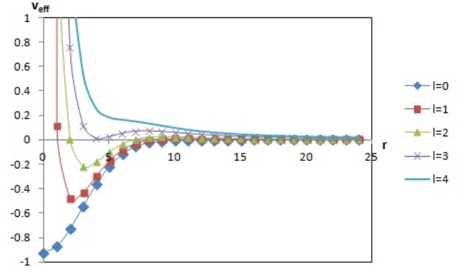
FIG. 8. The effect of the centrifugal term on the radial potential in the \mu \rightarrow 0 limit for the fitted erf-gau interaction [Eq. (19)].
