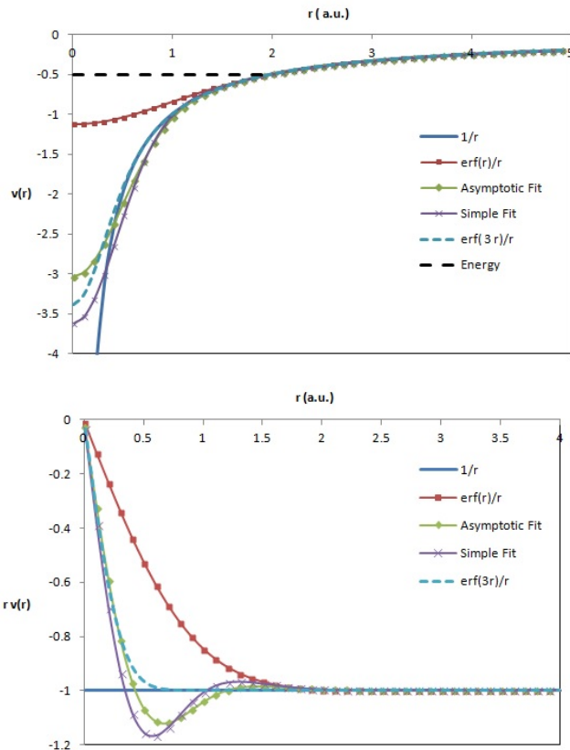
FIG. 3. Comparison between the Coulomb potential (solid line) and the model potentials: long-range (squares), asymptotic (diamonds), fitted (stars) and modified long-range potential (dashed line).
