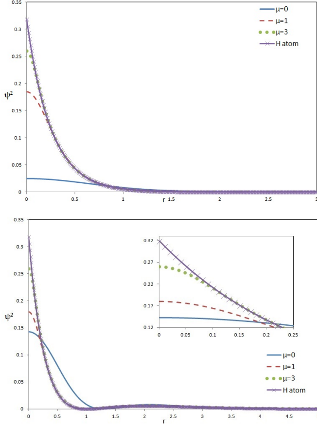
FIG. 9. The orbital densities |\psi_{1s}(r)|^2 (top) and |\psi_{2s}(r)|^2 (bottom) derived from the model Hamiltonian of Hydrogen, Eq. (8) with c = 0.923 + 1.568\mu , \alpha = 0.241 + 1.405\mu , using different values of \mu .
