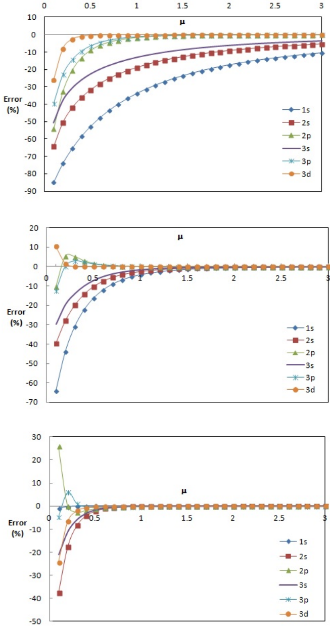
FIG. 4. Percentage errors in the eigenvalues of Hydrogen. From top to bottom: a) long-range \text{erf}(\mu r)/r , b) asymptotic [Eq. (16)], and c) fitted [Eq. (19)] potentials.
