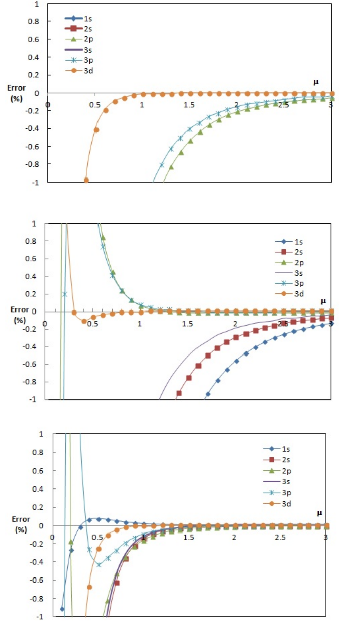
FIG. 5. Close-up of the percentage error of the eigenvalues of Hydrogen. As in Figure 4, the curves are, from top to bottom: a) long-range \text{erf}(\mu r)/r , b) asymptotic [Eq. (16)], and c) fitted [Eq. (19)] potentials.
