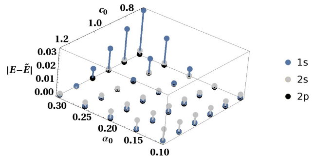
FIG. 1. The accuracy of the model potential spectrum with respect to the parameters c_0 and \alpha_0 . Energy errors (in %), for \mu = 1 .
