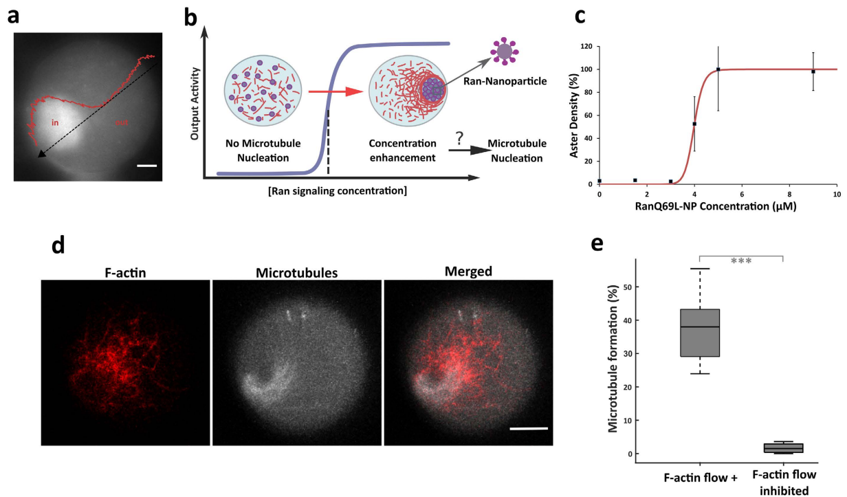
Figure 4. Signaling switch triggered by F-actin flow and by the active confinement of Ran-nanoparticles.
