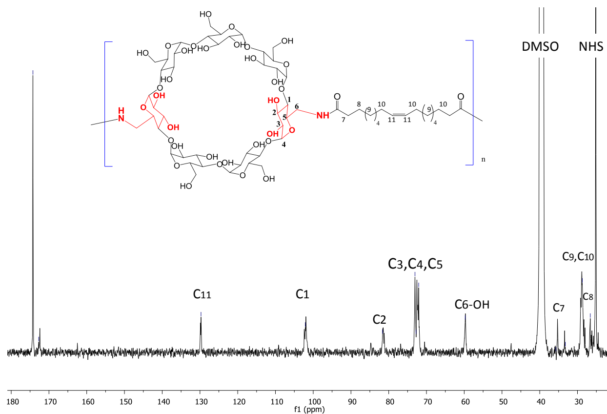
Figure 2: ^{13}\text{C} NMR of the polycondensate synthesized from the (Z) octadec-9-enedioic-N-hydroxysuccinimide ester and \beta\text{-CD}(\text{NH}_2)_2(\text{OH})_{19} in DMSO at 25°C.
