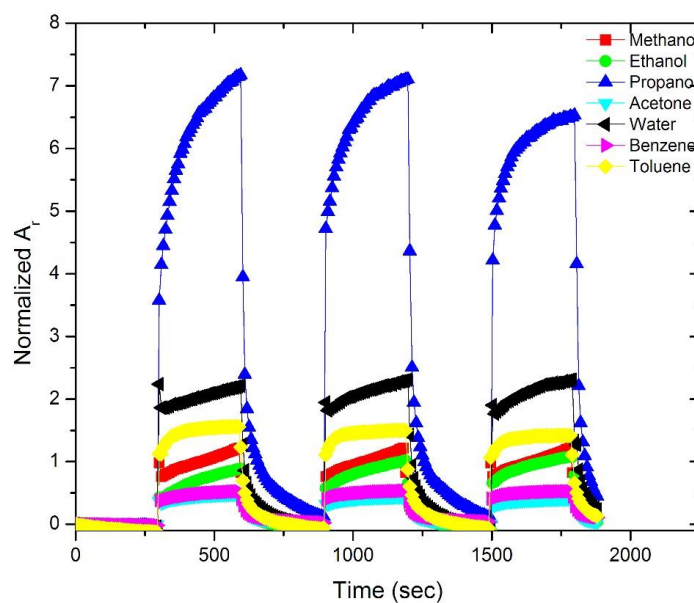
Figure 6. Effect of flow rate of different vapours on the amplitude A_r of branched polyamide based on \beta -CD(OH) 14 (NH 2 ) 7 -CNT sensor.
