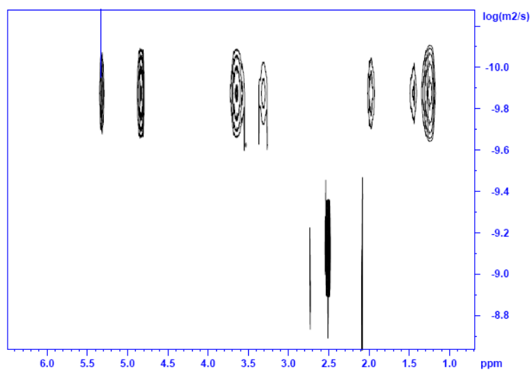
Figure 3: DOSY NMR spectrum of the polycondensate synthesized from the (Z) octadec-9-enedioic-N-hydroxysuccinimide ester and \beta -CD(NH 2 ) 2 (OH) 19 in DMSO at 25°C.
