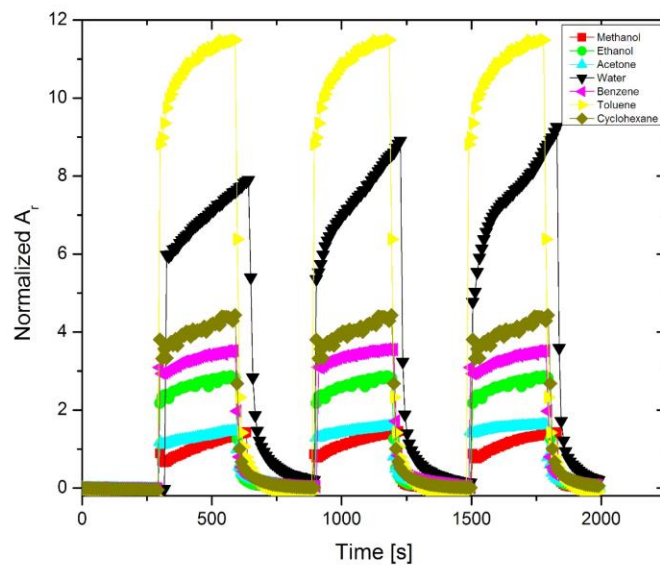
Figure 5. Effect of flow rate of different vapours on the amplitude A_r of linear polyamide based on \beta -CD(OBn) 19 (NH 2 ) 2 -CNT sensor.
