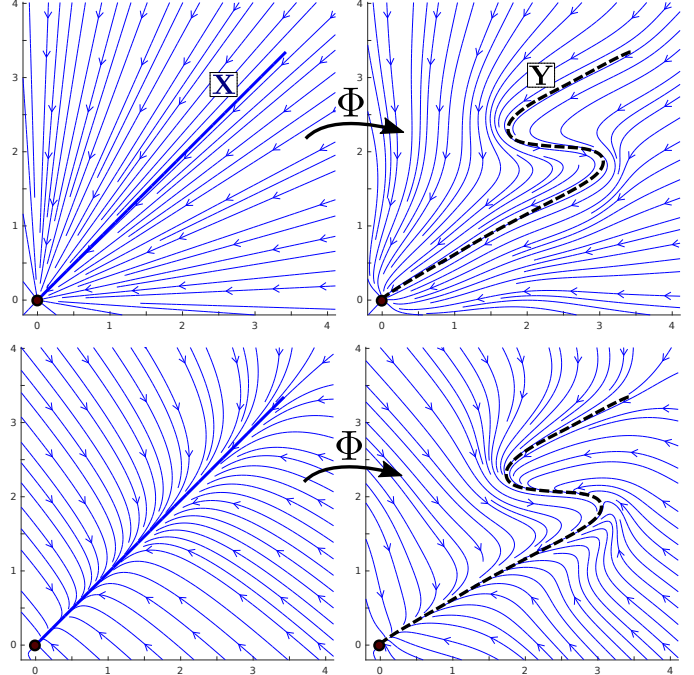
Figure 2: The diffeomorphism \Phi , that maps the trajectory \mathbf{X} onto \mathbf{Y} , transforms a stable DS with \mathbf{X} as a forward orbit into a stable DS with \mathbf{Y} as a forward orbit (top row). Using this property, we can modulate the initial vector field while keeping \mathbf{X} unchanged to obtain systems with different behaviors that all reproduce the demonstration \mathbf{Y} .
