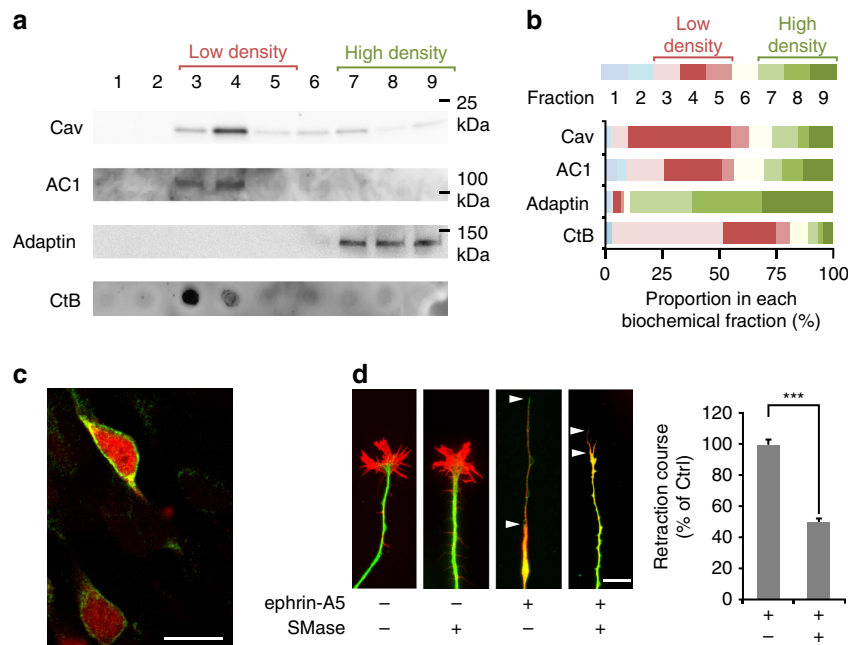
Figure 1 | Lipid rafts contain AC1 and are required for ephrin-A-induced axonal retraction. (a) AC1 fused to GFP and overexpressed in the developing retina is detected in fractions 3 and 4 after sucrose-density gradient fractionation of the plasma membrane. This coincides with the location of the lipid raft markers Caveolin-1 (Cav, enriched in fractions 3 and 4) and cholera toxin (CtB), a lipid raft marker that binds ganglioside M1, other gangliosides, and raft-targeted glycoproteins (enriched in fractions 3 and 4). AC1 is excluded from the fractions enriched in \beta -Adaptin (7–9), a marker of the non-raft fraction of the membrane. (b) Proportion of Caveolin, AC1, \beta -Adaptin and CtB expression found in each biochemical fraction. For each marker detected, the optical density (OD) of the bands in each fraction is quantified and normalized to the sum of the OD in all fractions. The proportion of the signal found in each fraction is shown. Each biochemical fraction is colour-coded. Red tones code for the low-density Caveolin- and CtB-enriched fractions (3–5), whereas green tones denote the high-density \beta -Adaptin-enriched fractions (7–9). Cav, Adaptin, AC1, CtB n = 3 independent experiments. (c) Overexpressing AC1 fused to GFP (green) in retinal neurons co-electroporated with mCherry (cytoplasmic localization, red) does not affect AC1 plasma membrane targeting. Scale bar, 10 \mu m. n = 3 experiments from independent cultures. (d) Altering lipid rafts integrity with SMase does not affect the morphology of growing RGC axons. Ephrin-A5 induces a collapse of RGC growth cones in vitro and a subsequent axonal retraction leaving a long trailing process (encompassed by the two arrowheads). SMase does not affect the collapse of the growth cone but reduces axon retraction measured as the length of the trailing process (between the two arrowheads). Scale bar, 10 \mu m. n \geq 360 axons per condition (ctrl n = 600 , SMase n = 360 ) from three independent cultures. Data are mean \pm s.e.m. *** P \leq 0.001 , Mann-Whitney test. Uncropped gels are provided in Supplementary Fig. 8.
