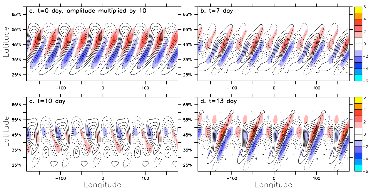
FIG. 3. Anomalous relative vorticity (contours; \text{CI}: 8 \times 10^{-6} \text{ s}^{-1} ) and momentum flux convergence (shadings; 10^{-4} \text{ m s}^{-2} ) at 200 hPa for the nonlinear simulation of the unstable normal mode with m = 5 at t = (a) 0 (b) 7, (c) 10, and (d) 13 days.
