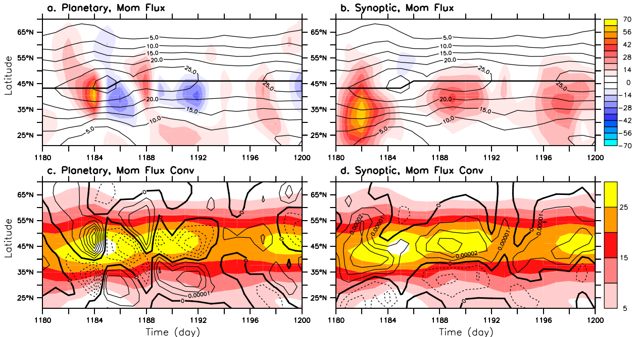
FIG. 6. (top) Vertically averaged momentum flux (shadings; \text{m}^2 \text{s}^{-2} ) and zonal wind (contours; \text{CI}: 5 \text{ m s}^{-1} ) as a function of time and latitude from t = 1180 to 1200 days of the long-term simulation. (bottom) Vertically averaged momentum flux convergence (contours; \text{CI}: 10^{-5} \text{ m s}^{-2} ) and zonal wind (shadings; \text{m s}^{-1} ) as a function of time and latitude. (a),(c) Planetary wave and (b),(d) synoptic wave.
