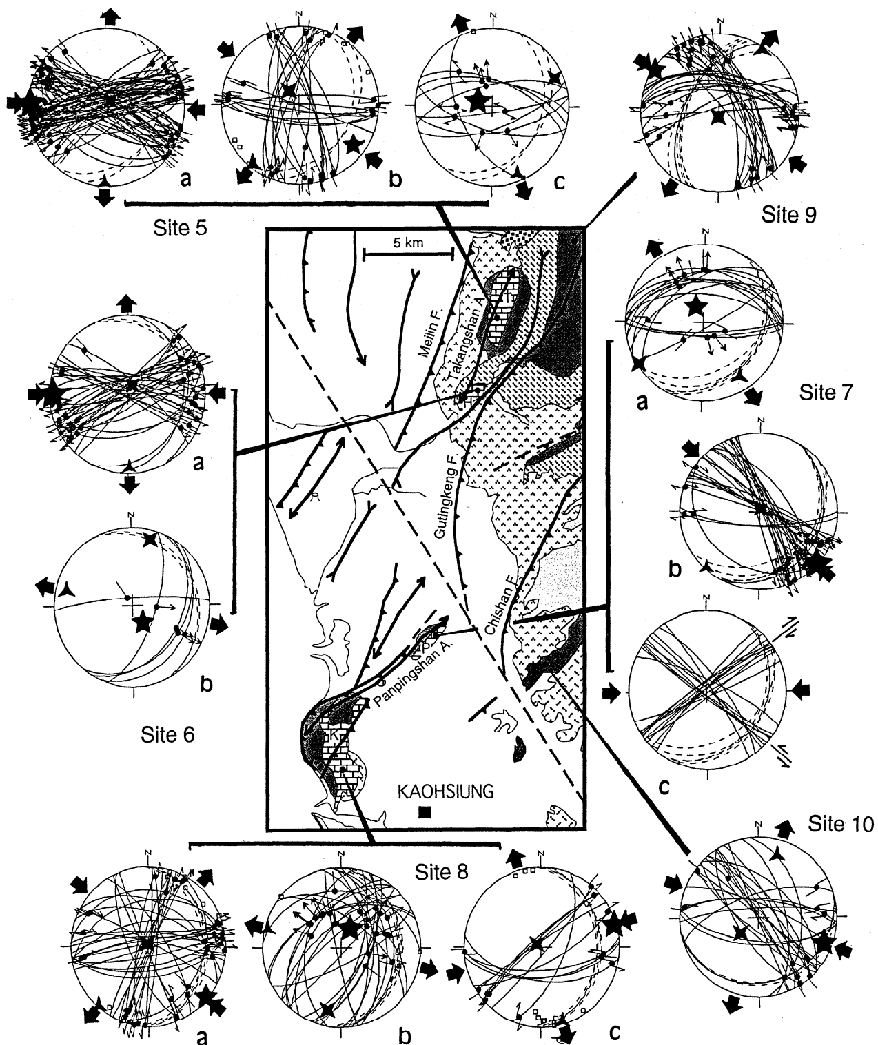
Figure 8. Results of stress reconstruction based on fault slip analysis in the vicinity of the Takangshan and Panpingshan anticlinics. The map is part of that of Figure 2 (Longitude: 120^{\circ}15' - 120^{\circ}25' ; Latitude: 22^{\circ}35' - 22^{\circ}55' ) and uses the same key as in Figures 2 and 7. Small open squares in diagrams represent poles to tension gashes.
