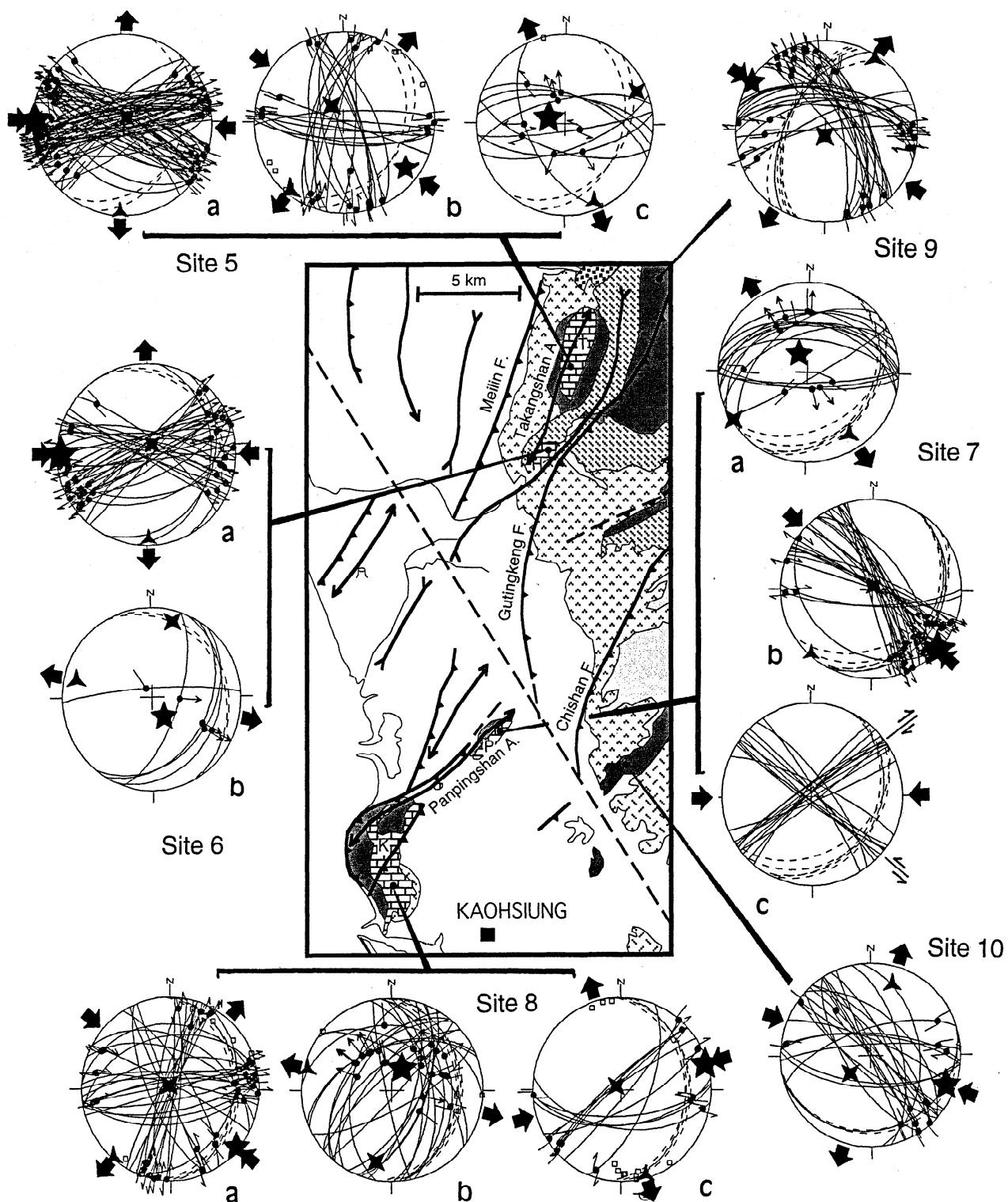
Figure 8. Results of stress reconstruction based on fault slip analysis in the vicinity of the Takangshan and Panpingshan anticlinics. The map is part of that of Figure 2 (Longitude: 120^{\circ}15' - 120^{\circ}25' ; Latitude: 22^{\circ}35' - 22^{\circ}55' ) and uses the same key as in Figures 2 and 7. Small open squares in diagrams represent poles to tension gashes.
