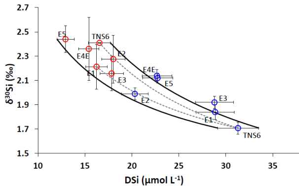
Figure 5. Potential mixing curves between TNS6-WW and the different meander ML water masses; WW is in blue and the ML is in red. The two end-members are identified by black curves. The two grey dashed lines represent the mixing curves between TNS6-WW and TNS6-ML and between TNS6-WW and E1-ML, which may explain the Si properties of E1-WW and E2-WW respectively. The ML averages and error bars were calculated based on the median values and interquartile range for each station, while the “central value” was defined using the salinity threshold method for WW.
