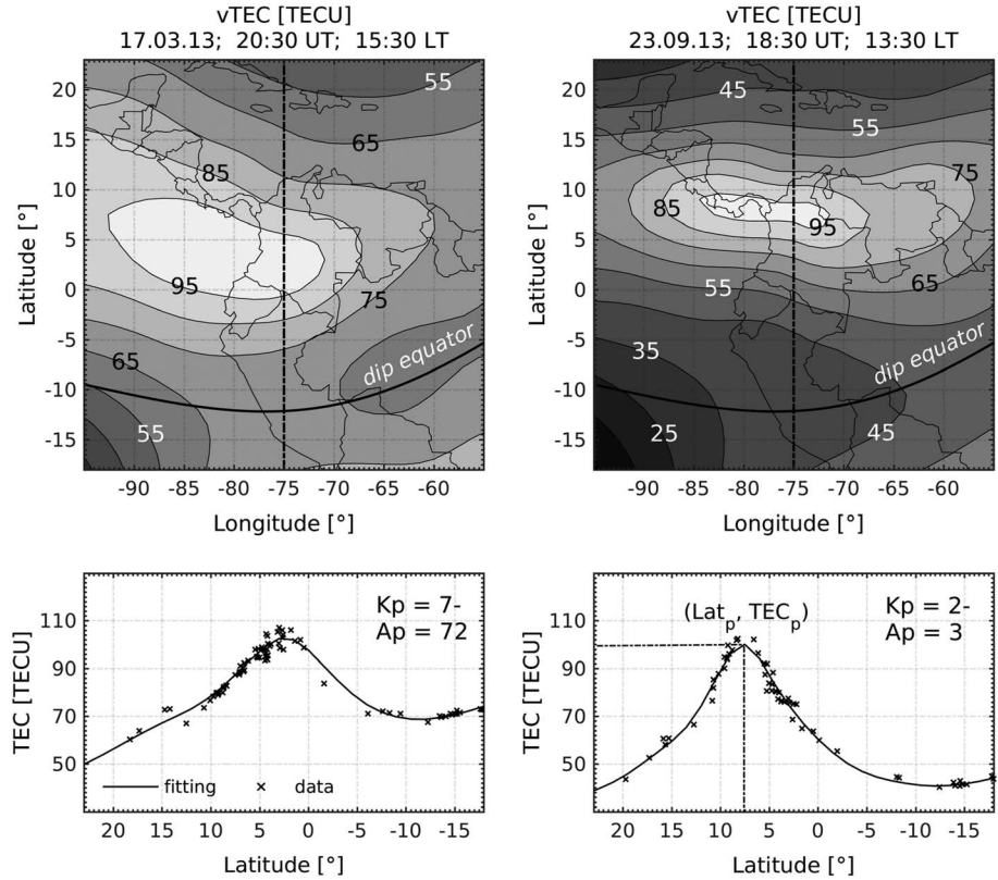
Figure 3. (top) Daytime maximum vTEC maps of the northern crest of the EIA over South America on 17 March and 23 September 2013. (bottom) The corresponding vTEC meridional cross sections at 75°W.
