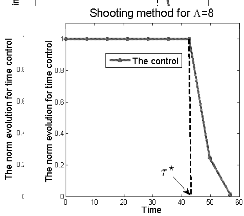
FIGURE 3 – The norm evolution L^2 for time control with \Lambda = 8
