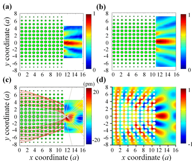
FIG. 4. (a) Experimental and (b) numerical distribution of the normalized maximum u_z behind the acoustic lens at 7.2 MHz, together with (c) experimental and (d) numerical snapshots of the near field focusing at 7.2 MHz. (c) The gray solid lines and the red dashed lines are for the ray trajectories with |k_y| < |k_B| and |k_y| > |k_B| , respectively.
