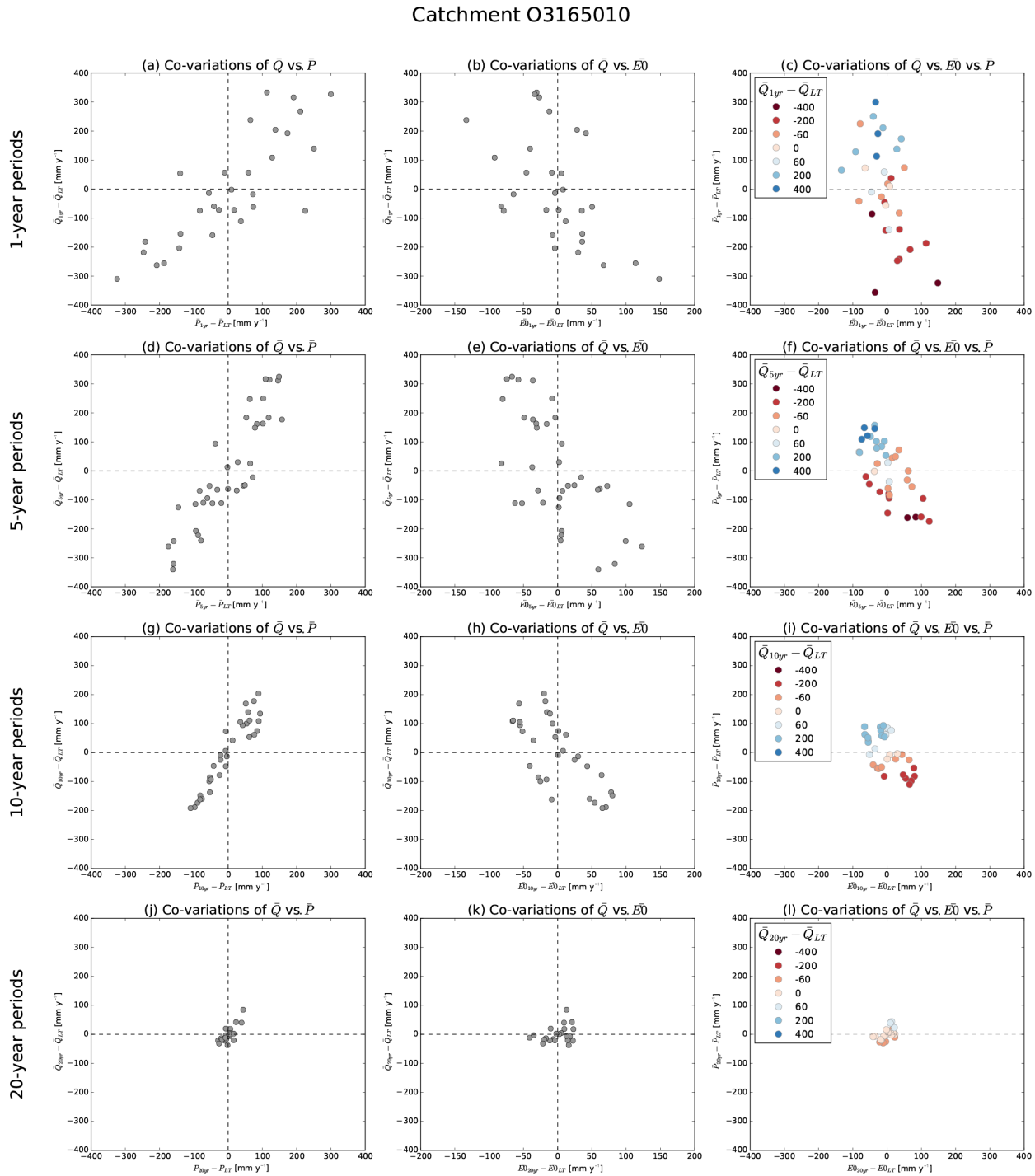
Figure 5. Impact of period length on the streamflow elasticity graphs for an empirical (data-based) assessment. The graphs present from left to right \Delta Q vs. \Delta P , \Delta Q vs. \Delta E_0 , and \Delta Q (in colors) vs. \Delta P and \Delta E_0 . LT stands for long term (entire period).
