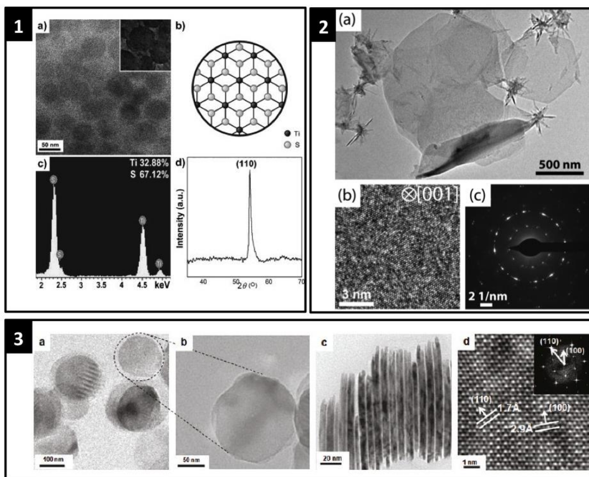
Figure 30: 1- (a) TEM image showing top view of 50-nm TiS 2 nanodisks, (b) structural diagram, (c) EDS spectrum, and (d) PXRD pattern. From ref.240. Copyright 2008 by John Wiley & Sons, Inc. Reprinted by permission of John Wiley & Sons, Inc. 2- (a) Low- and (b) high-resolution TEM images of TiS 2 NSs. (c) SAED pattern of TiS 2 NSs stacked atop each other. Adapted with permission from ref.241. Copyright (2012) American Chemical Society. 3- TEM images of TiS 2 discs: (a, b) Low-resolution and magnified images of TiS 2 disc nanocrystals (c) Side view of TiS 2 discs stacked together. (d) HRTEM image and (inset) FFT pattern of TiS 2 . Adapted with permission from ref.242. Copyright (2011) American Chemical Society.
