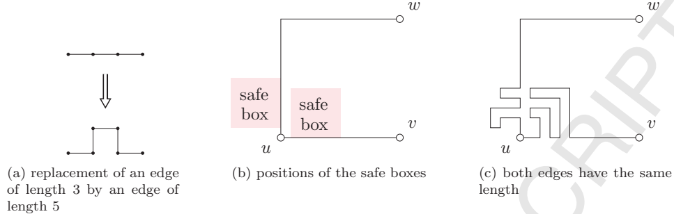
Figure 2: Construction of the orthogonal embedding
