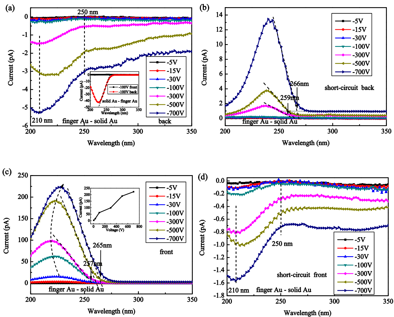
Figure 6. Comparison of photocurrent spectra for samples (a) when a negative voltage is applied to the back electrode, (b) after the removal of a negative voltage from the back electrode, (c) when a negative voltage is applied to the front electrode, and (d) after the removal of the negative voltage from the front electrode. The inset of figure 6 (a) shows the photocurrent spectra for solid Au - finger Au sample, and the inset of figure 6 (c) shows the dependence of peak amplitude on the applied voltage.
