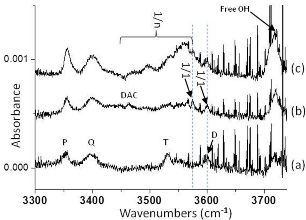
Figure 2: Jet-AILES FTIR spectrum in the OH bonded and free stretching region of water containing complexes recorded at 0.5 \text{ cm}^{-1} resolution for different dilutions of the ternary mixture DAC/H 2 O/Ar: (a) 0/8/1000, (b) 8/8/1000, (c) 8/16/1000. The notation D stands for water dimer, T for water trimer, Q for water tetramer and P for water pentamer.
