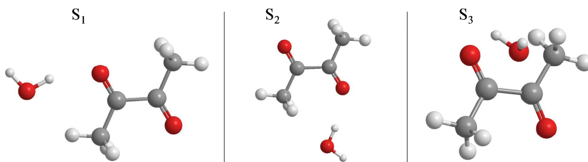
15 16 17 18 19 20 21 22 23 24 25 26 27 28 29 30 31 32 33 34 35 36 37 38 39 40 41 42 43 44 45 Figure 1: The three isomers for the 1/1 complex optimized at MP2/AVTZ level of theory.
