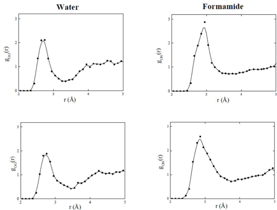
Figure 2. Left panel: anionic oxygen-water oxygen radial distribution functions of the 2',3' cyclic nucleotide model (upper panel) and of its 3',5' counterpart (lower panel) in water computed at 363 K. Right panel: anionic oxygen-formamide nitrogen radial distribution functions of the 2',3' cyclic nucleotide model (upper panel) and of its 3',5' counterpart (lower panel) in formamide at 363 K.
