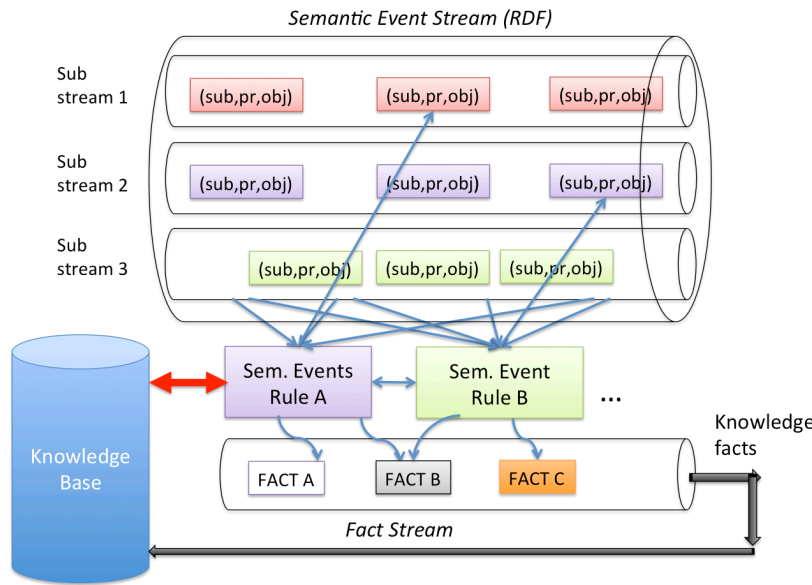
Fig. 2. Mapping Semantic Events to Knowledge Facts
