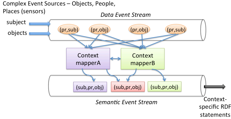
Fig. 1. Mapping Data Events to Semantic Events
