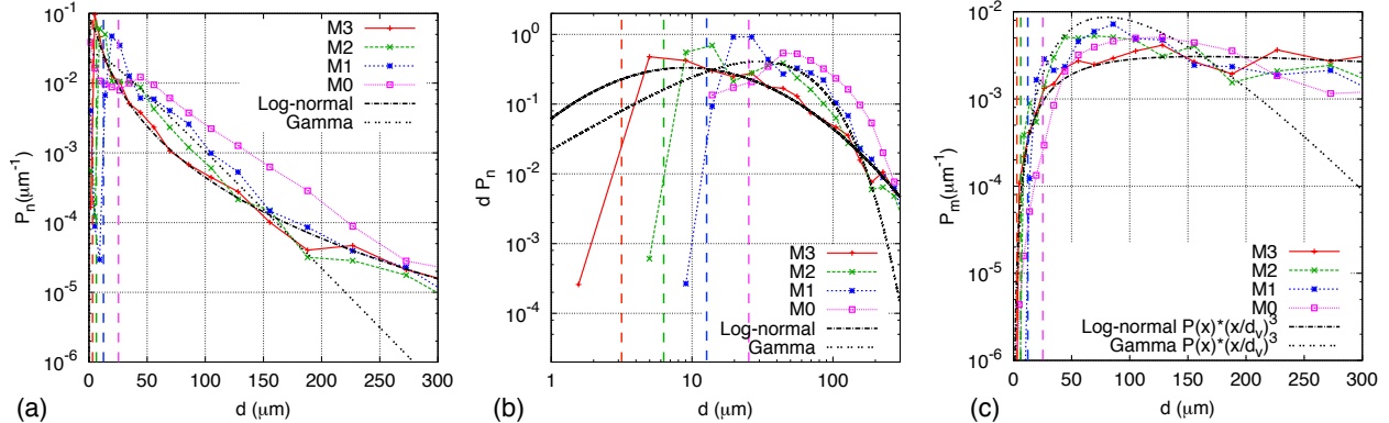
FIG. 13. Comparison of droplet (a, b) number and (c) mass PDF profiles with the log-normal and gamma distribution functions. The bin width increases with d by a constant ratio 1.2 from 3.125 \mu\text{m} . The mesh size for different cases are indicted by vertical dash lines with corresponding colors.
