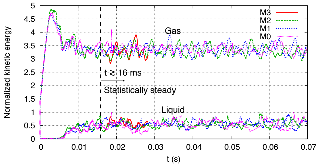
FIG. 2. Temporal evolution of mean kinetic energy of gas and liquid over the computational domain for different meshes. The kinetic energy is normalized by U_g^2 .
