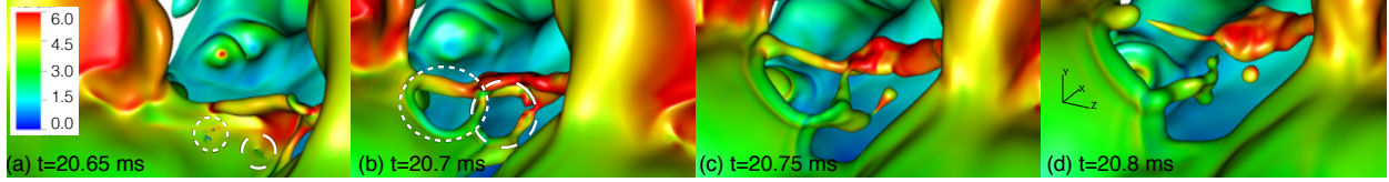
FIG. 9. Ligaments formation due to holes in a liquid sheet. The color on the interface indicates the streamwise velocity.
