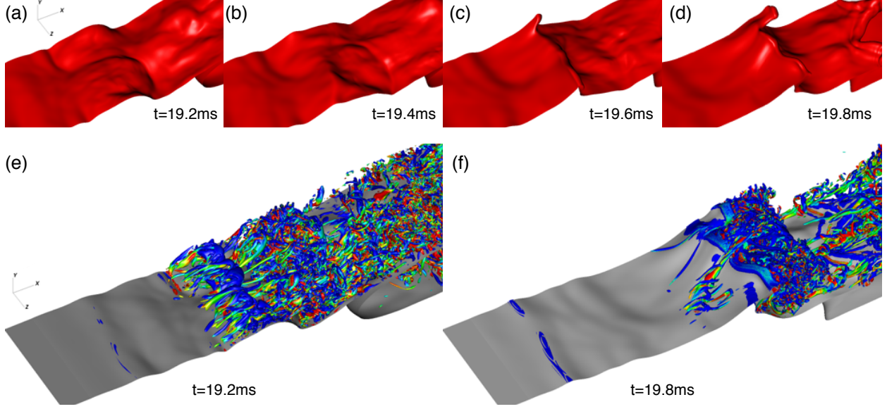
FIG. 4. Development of a fully 3D interfacial wave: (a)-(d) time snapshots of the interface and (e)-(f) turbulent vortical structures in the gas-liquid mixing layer (visualized by the \lambda_2 criterion).
