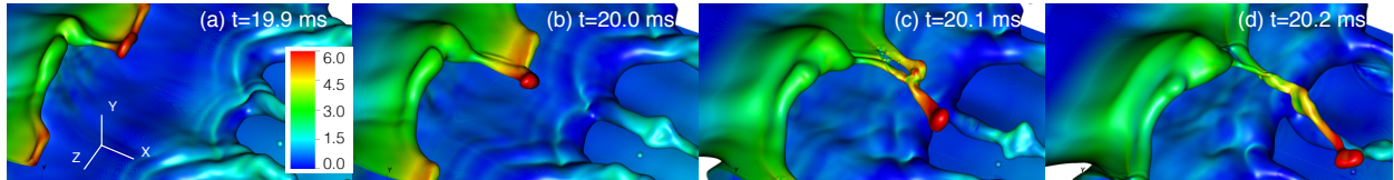
FIG. 8. Ligaments formation due to fingering at the tip of a liquid sheet. The color on the interface indicates the streamwise velocity.
