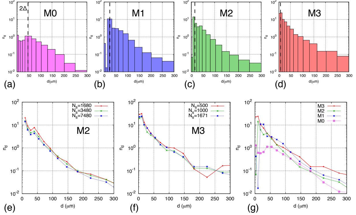
FIG. 12. The size distribution of droplet number. Histograms of n_d for different meshes are shown in (a)-(d). The bin width increases with d by a constant ratio 1.2 from 6.25 \mu\text{m} . The size distribution of n_d for different sample number is shown in (e) and (f) for the M2 and M3 meshes, directly. The comparison of n_d for different meshes is shown in (g). The vertical dash lines in (a)-(d) indicate d = 2\Delta for different meshes.
