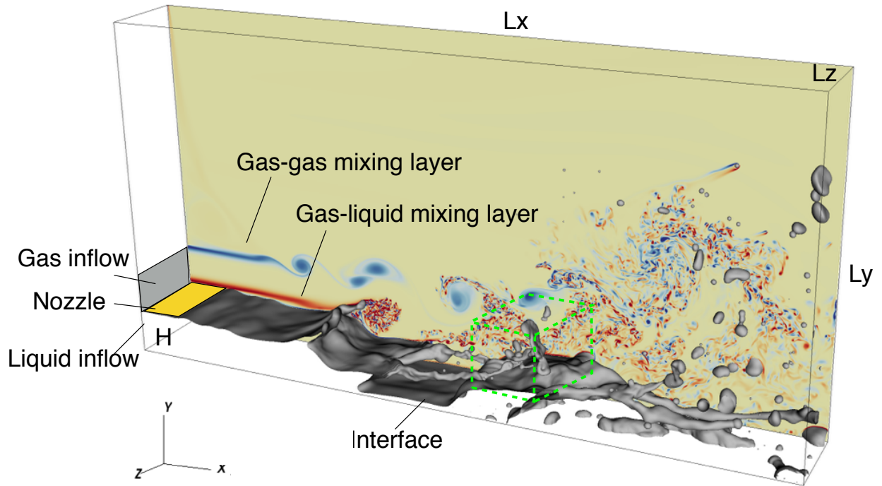
FIG. 1. Spray formation in a gas-liquid mixing layer. The z -vorticity is shown on the backplane. The sampling region for droplets statistics is indicated by green lines.
