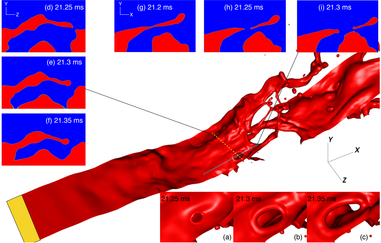
FIG. 10. Evolution of a hole formed in a liquid sheet. (a)-(c) A closeup a the hole expansion. Liquid volume fraction (red) at y - z and y - x planes cutting through the holes are also shown in (d)-(f) and (g)-(i), respectively.
