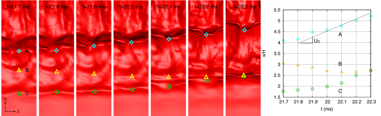
FIG. 5. Interfacial waves interaction (results by M2 mesh). Symbols indicate locations of the wave crests at plan z = H . The Dimotakis speed (black dashed line) is plotted for comparison.
