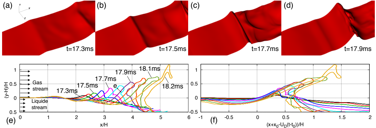
FIG. 3. Development of a quasi-2D interfacial wave, forming a liquid sheet: (a)-(d) time snapshots of the interface; interface profiles at plane z = H with (e) original scale and (f) x -axis scaled by the Dimotakis speed U_D .
