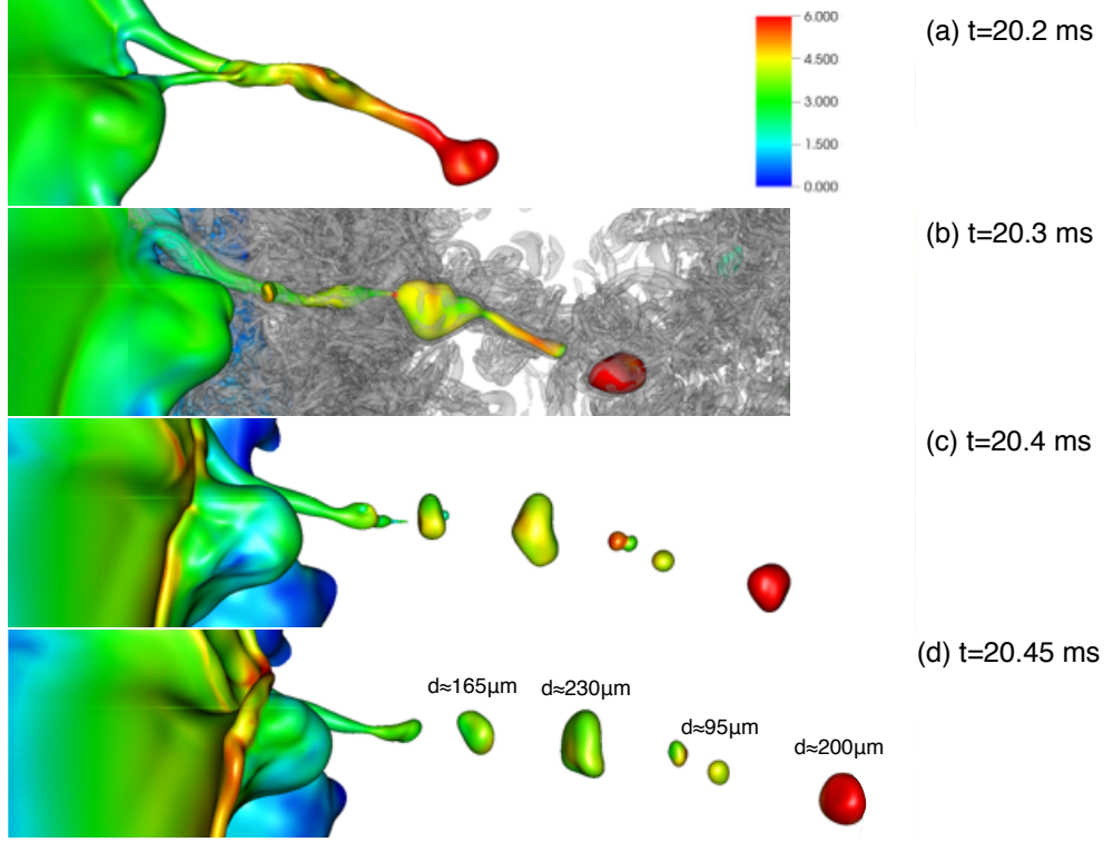
FIG. 11. Droplets generation due to ligament breakup. The turbulent vortices surrounding the ligament is plotted in (b) by the \lambda_2 criterion.
