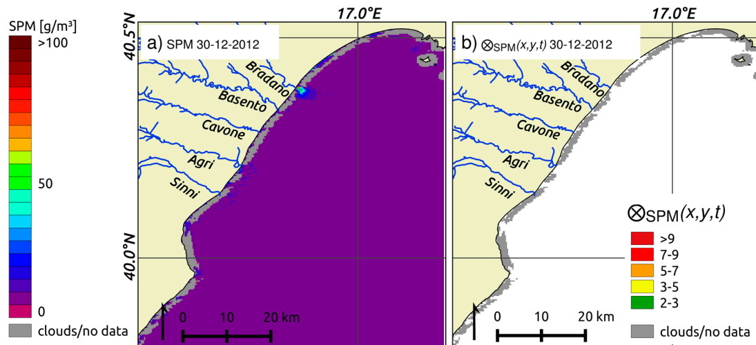
Figure 10. (a) SPM and (b) \otimes \text{SPM}(x, y, t) maps of 30 December 2012, where no anomaly is detected by RST methodology.
