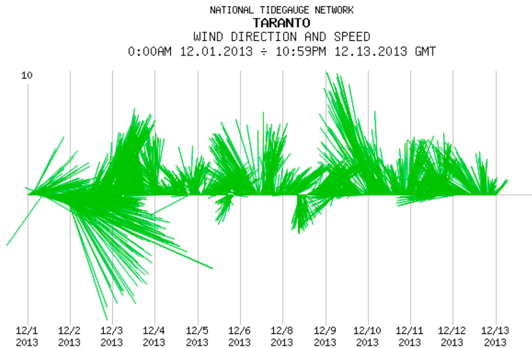
Figure 3. The registered wind intensity (m/s) and direction measured every 10 min in the 1–13 December 2013 period at the Taranto station (data from [35]).
