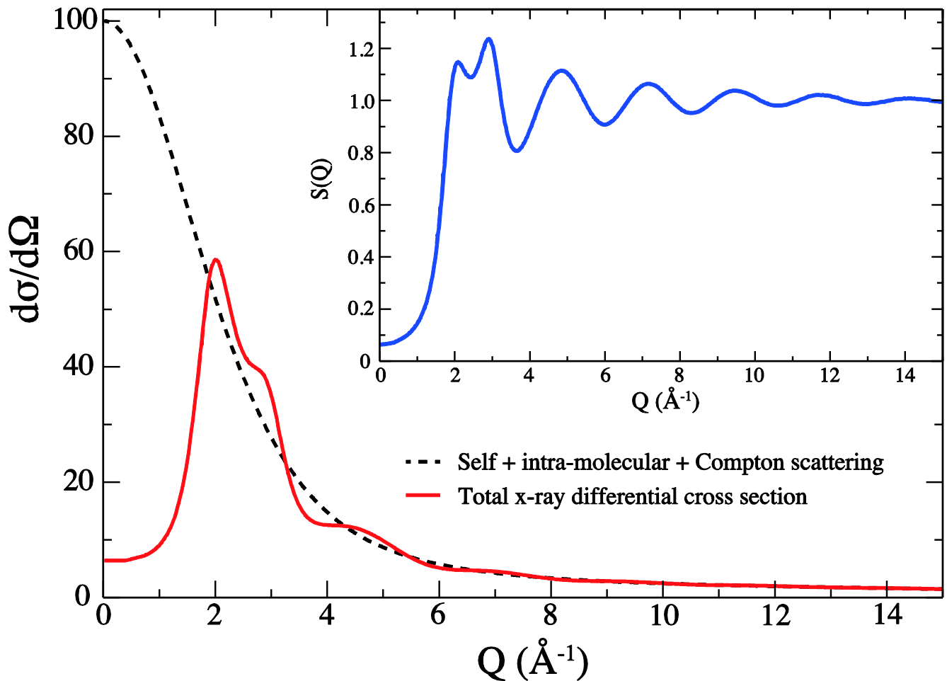
Figure 3. Total x-ray differential scattering cross section d\sigma/d\Omega(Q) of water 11 (full red line). The sum of self-scattering, intra-molecular scattering and Compton scattering is indicated by the dashed black line. The total coherent x-ray scattering cross section, called the total structure factor S(Q) (inset, blue line), is obtained after subtraction of the self, intra-molecular and Compton scattering contribution
