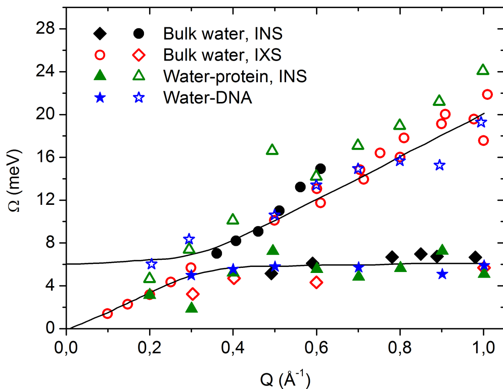
Figure 12. Dispersion curves of bulk water and water at the interface with biomolecules. The excitation energies of bulk water were measured with both INS (black closed rhombuses 162 , closed black circles 163 ) and IXS (red open rhombuses 164,165 , red open circles 166 ). The excitation energies of water at the interface with RNase protein 167 (closed and open green triangles, for the low- and high-energy branches respectively) and DNA 168 (closed and open blue stars, for the low- and high-energy branches respectively) were measured by INS. The continuous line represents the two-mode interaction model 169 .
