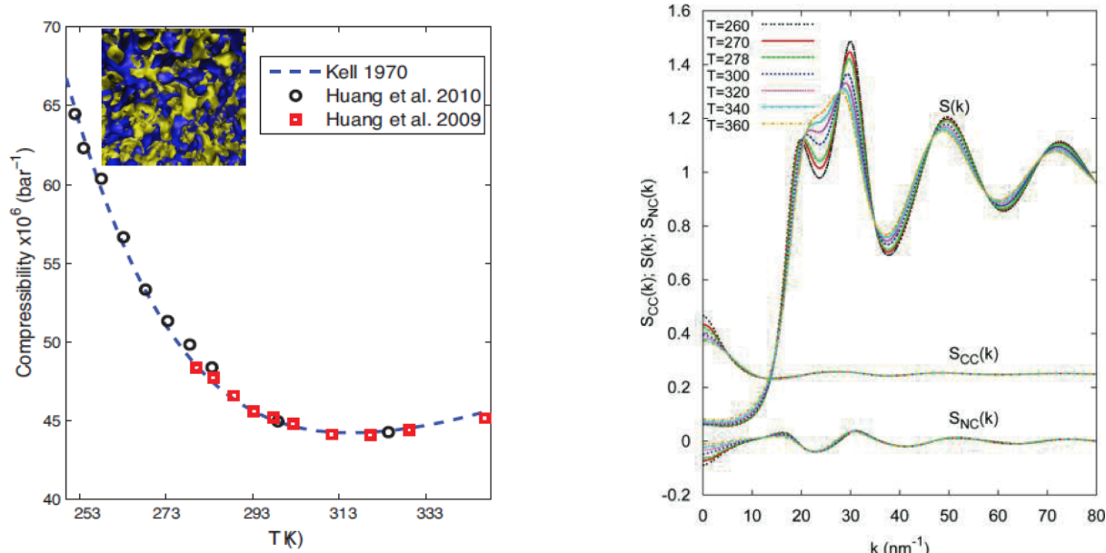
Figure 5. (left) Isothermal compressibility determined from either macroscopic thermodynamic measurements (dashed line) 53 or extracted from the SAXS data (circles and squares) 49, 50 . (Right) Concentration-concentration ( S_{CC}(k) ), density-density ( S(k) ) and density-concentration ( S_{NC}(k) ) 56 . (Inset): Isosurfaces at 253 K of high-density fields (yellow) and high tetrahedrality (blue) from TIP4P/2005 simulations 57 . The length of the box is \sim 106 \text{ \AA} . Reproduced from ref. 58 .
