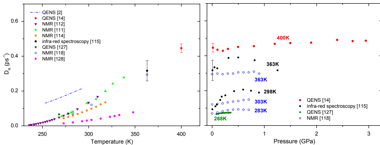
Figure 10. Rotational diffusion coefficient for liquid water as a function of temperature (left panel) and of pressure (right panel), as derived from different techniques. 2, 14, 112, 111, 114, 115, 127, 118, 128
