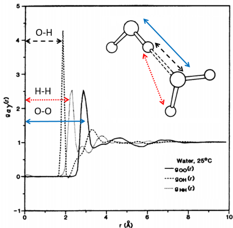
Figure 1. Adapted from 26 . Partial pair distribution functions obtained from neutron diffraction and H-D substitution.
