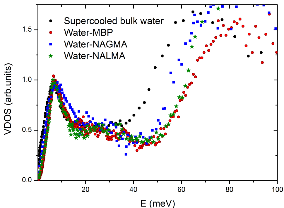
Figure 11. Vibrational density of states of supercooled water measured on the IN6 spectrometer (Institut Laue-Langevin, Grenoble) 136 and water at the interface with maltose binding protein (MBP) 16 , 147 , NALMA and NAGMA molecules 17 , measured on the IN5 spectrometer (Institut Laue-Langevin, Grenoble). The VDOS curves have been normalised to the first inelastic peak at 6 meV.
