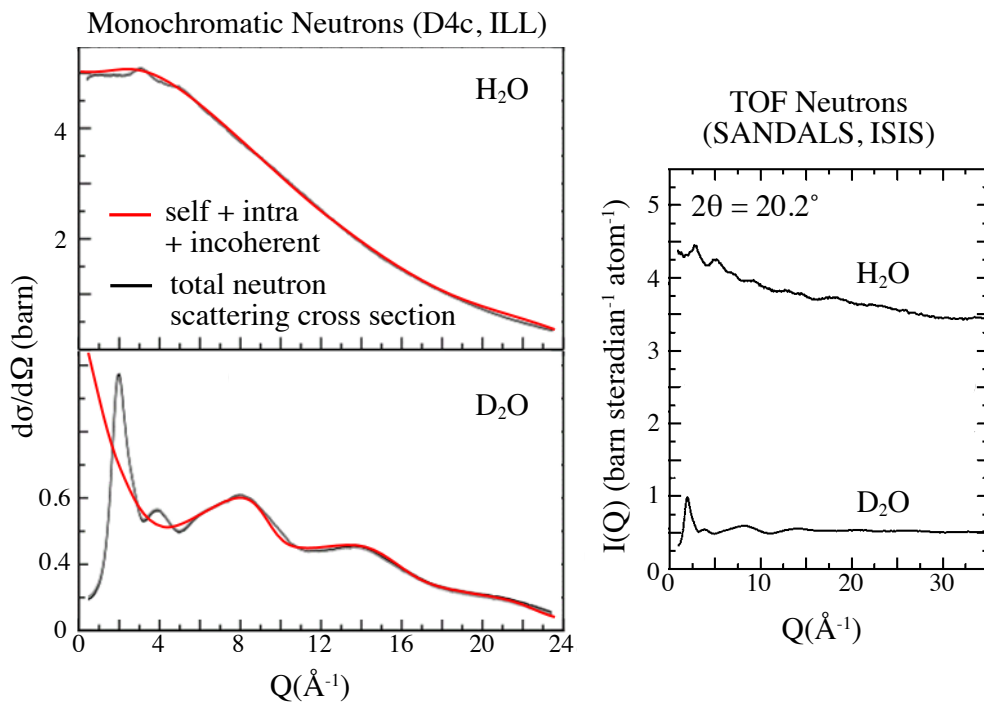
Figure 2. Total differential scattering cross sections of pure H 2 O and pure D 2 O water as measured by two different neutron scattering techniques. Left: monochromatic neutrons ( \lambda=0.5\text{\AA} ) using the reactor source ILL (Grey lines). The red line corresponds to the sum of self plus intramolecular plus incoherent contributions (see chapter 2.1 for details). Right: time-of-flight neutron diffraction (TOF) at the pulsed neutron source ISIS which uses a wide band of incident neutron energies ( \lambda \sim 0.1\text{-}3\text{\AA} ) (Black lines).
