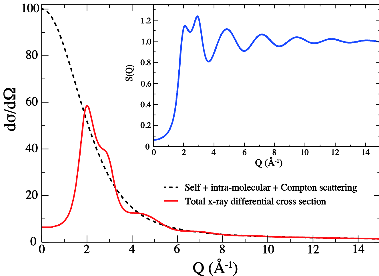
Figure 3. Total x-ray differential scattering cross section d\sigma/d\Omega(Q) of water 11 (full red line). The sum of self-scattering, intra-molecular scattering and Compton scattering is indicated by the dashed black line. The total coherent x-ray scattering cross section, called the total structure factor S(Q) (inset, blue line), is obtained after subtraction of the self, intra-molecular and Compton scattering contribution
