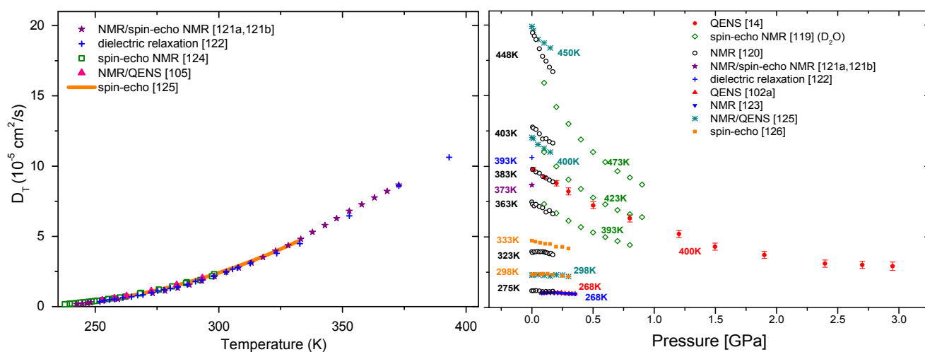
Figure 9. Translational diffusion coefficient for liquid water as a function of temperature (left panel) and of pressure (right panel), as derived from different techniques. 14, 119, 120, 121, 122, 102a, 123, 124, 105, 125, 126.
