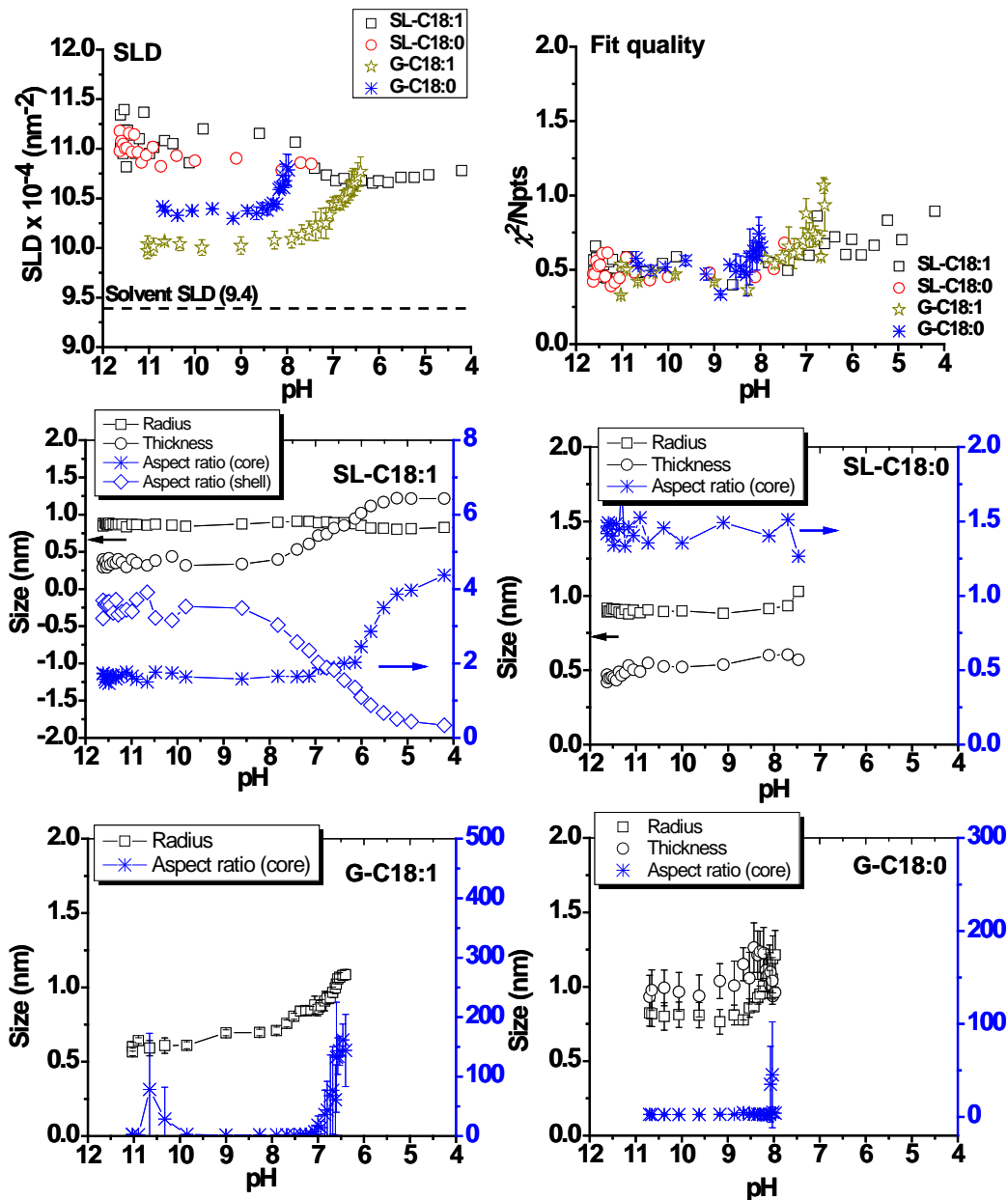
Figure 5 – pH-dependent evolution of the core-shell ellipsoid of revolution model fit parameters. SLD: evolution of the fitted scattering length density; Fit quality: evolution of the \chi^2/Npts quality control parameter. SL-C18:1, SL-C18:0, G-C18:1, G-C18:0 panels: evolution of the core radius, shell thickness (where applicable), core and shell (where applicable) aspect ratios for the core-shell ellipsoid of revolution form factor model (the details of the model are given in the Supporting Information).
