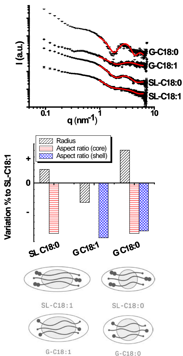
Figure 2 – SAXS data (with error bars) corresponding to both sophorolipids and glycolipids (0.5 w%) at \text{pH } 11.0 \pm 0.3 . The red curves correspond to the fit performed using a core-shell ellipsoid of revolution form factor model. The fitting procedure for this system has been outlined in the Supporting Information. The histogram shows the relative variation of the most significant fitting parameters (Radius, aspect ratio (core, shell), keeping all other constant, for the SL-C18:1, G-C18:1 and G-C18:0 samples and with respect to the reference compound, SL-C18:1. The modeled ellipsoids structures for each glycolipid are given on the bottom of the figure.
