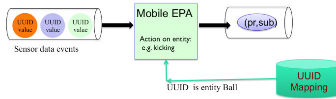
Fig. 1. Semantic annotation from raw sensor data
