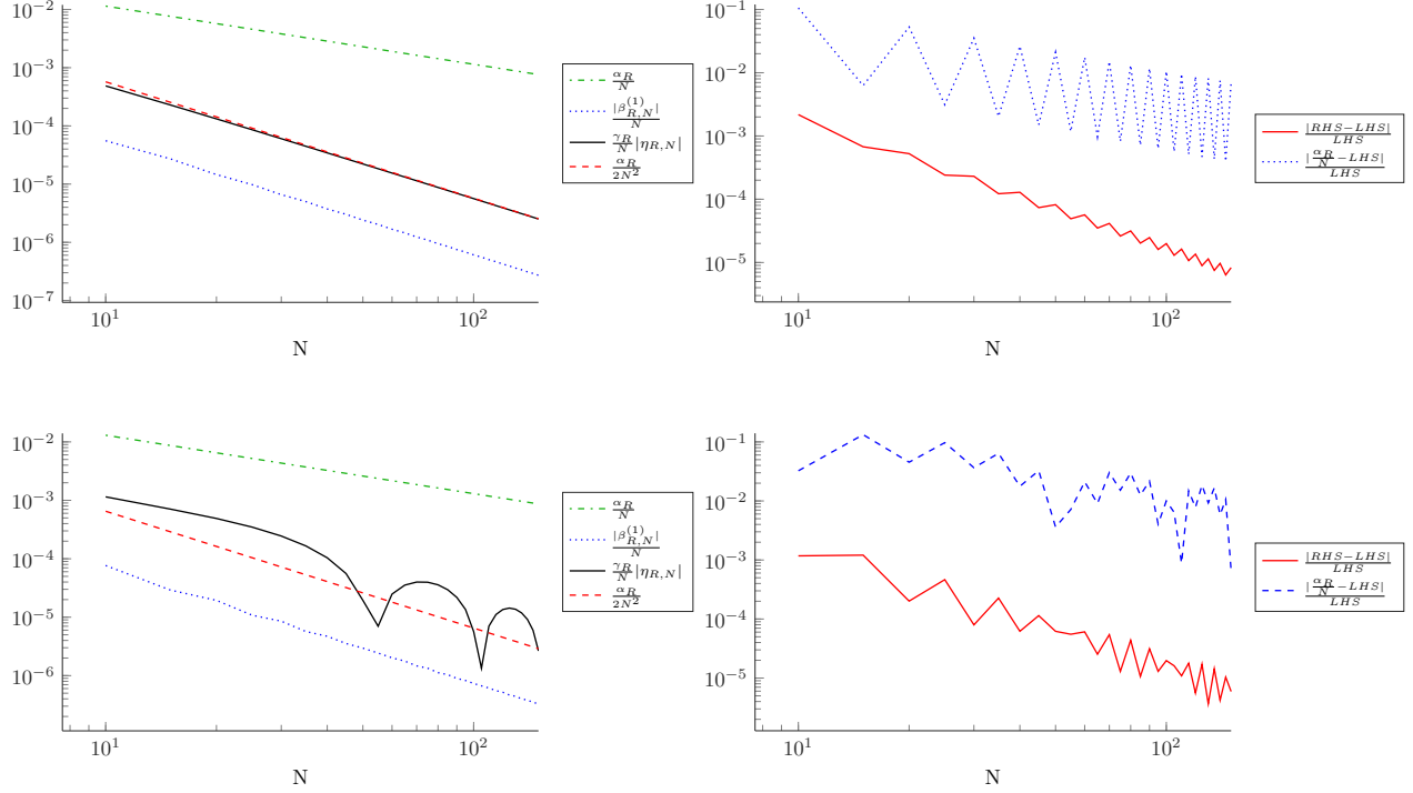
Figure 6. Convergence plots of the four quantities \frac{\alpha_R}{N} , \frac{\alpha_R}{2N^2} , \frac{|\beta_{R,N}^{(1)}|}{N} , and \frac{\gamma_R}{N}|\eta_{R,N}| (left) and plots of \frac{(|\frac{\alpha_R}{N} - \frac{\alpha_R}{2N^2} + \frac{\beta_{R,N}^{(1)}}{N} + \frac{\gamma_R}{N}\eta_{R,N}| - (E_{R,N} - E_R))}{E_{R,N} - E_R} and \frac{|\frac{\alpha_R}{N} - (E_{R,N} - E_R)|}{E_{R,N} - E_R} (right). Top: z_1 = z_2 = 1, R = 0.3 . Bottom: z_1 = z_2 = 1, R = 0.09 .
