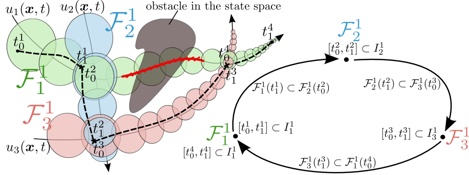
Fig. 2. Run of a funnel system with three control funnels: r = ((\mathcal{F}_1^1, v_0^1), (\mathcal{F}_1^1, v_1^1), (\mathcal{F}_2^1, v_0^2), (\mathcal{F}_2^1, v_2^2), (\mathcal{F}_3^1, v_0^3), (\mathcal{F}_3^1, v_3^3), (\mathcal{F}_4^1, v_0^4), (\mathcal{F}_4^1, v_1^4)) , with: \forall 1 \leq i \leq 4, v_0^i(c_t) = t_0^i, v_1^i(c_t) = t_1^i, v_0^i(c_h) = 0, v_1^i(c_h) = t_1^i - t_0^i, v_1^i(c_g) = v_0^i(c_g) + v_1^i(c_h) , and v_0^1(c_g) = 0 , and \forall 2 \leq i \leq 4, v_0^i(c_g) = v_1^{i-1}(c_g) .
