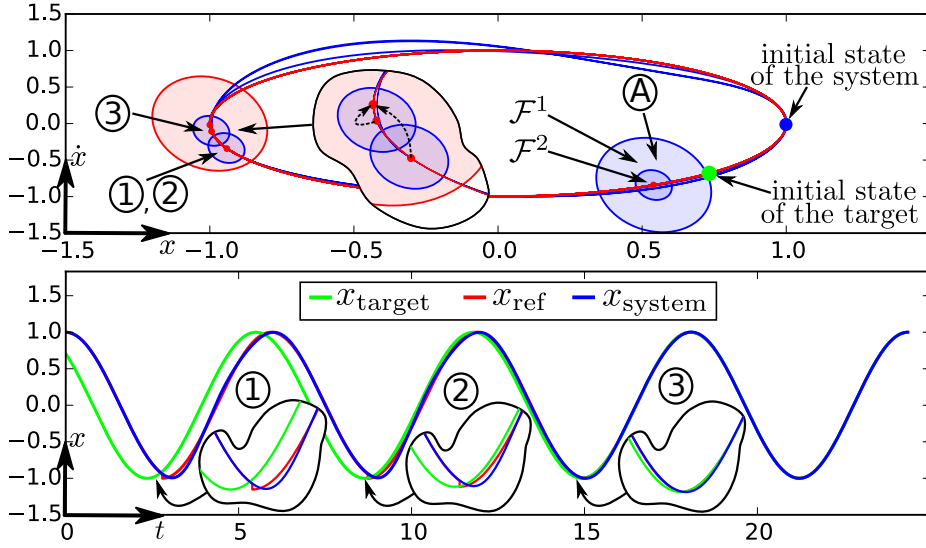
Fig. 5. The reactive controller performs three switching transitions to exactly adjust its signal to that of the target signal.
