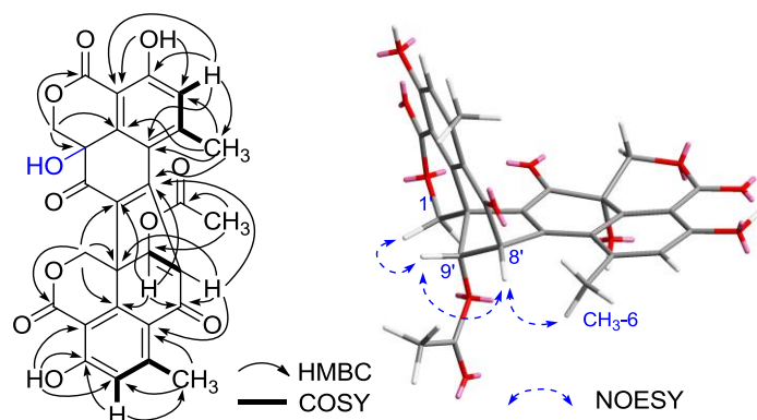
Figure 1. Key HMBC, COSY and NOESY correlations of 1 .
