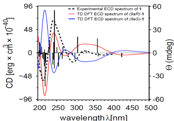
Figure 2. Comparison of the calculated and experimental ECD spectra of 1 .
