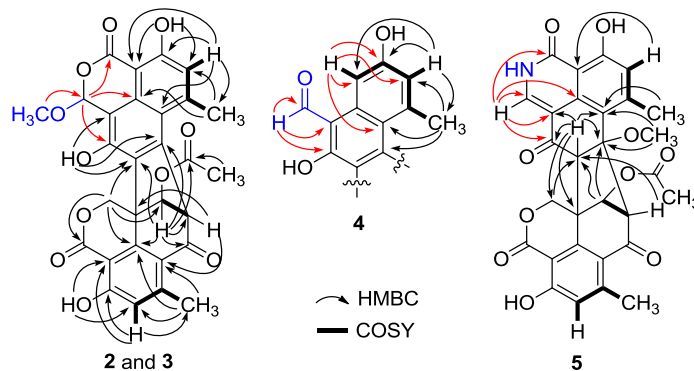
Figure 3. Key HMBC correlations of bacillisporins F–H ( 2 – 5 ).
