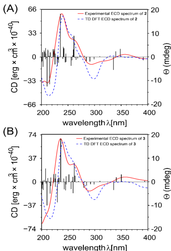
Figure 4. Comparison between calculated and experimental ECD spectra: (A) compound 2 and (B) compound 3 .
