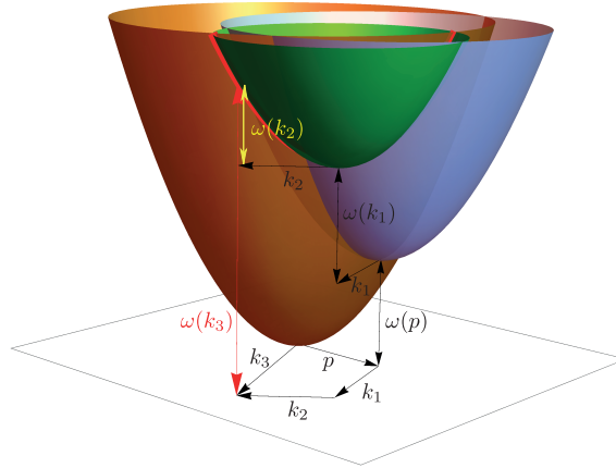
Figure 1: The plot represents the intersection of the surfaces for a parabolic dispersion relation \omega(\mathbf{k}) = \frac{1}{2}|\mathbf{k}|^2 . This is the case of a decaying situation in the 3 \leftrightarrow 1 .
