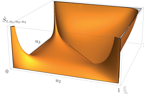
Figure 3: The bound S -matrix \hat{S}_{\omega_p\omega_1\omega_2\omega_3} as a function of the dimensionless variables u_2 = \omega_2/\omega_p , u_3 = \omega_3/\omega_p , and here it is understood that u_1 = \omega_1/\omega_p and u_1 = u_2 + u_3 - 1 if u_2 + u_3 \geq 1 , u_1 = 1 - (u_2 + u_3) if u_2 + u_3 < 1 , and, finally, u_1 = 0 if u_2 + u_3 = 1 . Notice that \hat{S}_{\omega_p\omega_1\omega_2\omega_3} = 0 at the line \omega_2 + \omega_3 = \omega_p .
