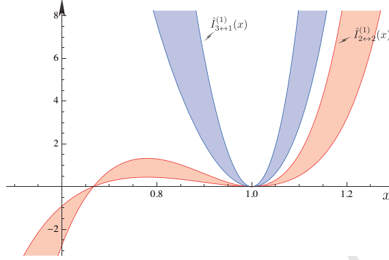
Figure 4: The bounds of the collisional integrals \hat{I}_{2\leftrightarrow 2}^{(1)}(x) and \hat{I}_{3\leftrightarrow 1}^{(1)}(x) as functions of x . The shadow domains represent the possible values of the exact collisional integrals I_{2\leftrightarrow 2}^{(1)}(x) and I_{3\leftrightarrow 1}^{(1)}(x) .
