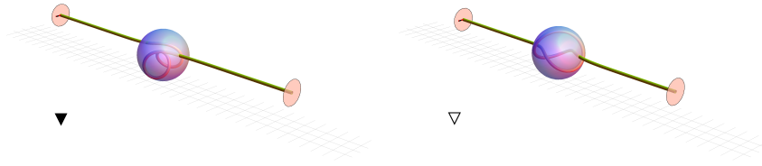
Fig. 8 3D configurations corresponding to the up and down triangles on the post-buckling diagram of Figures 3 and 4.
