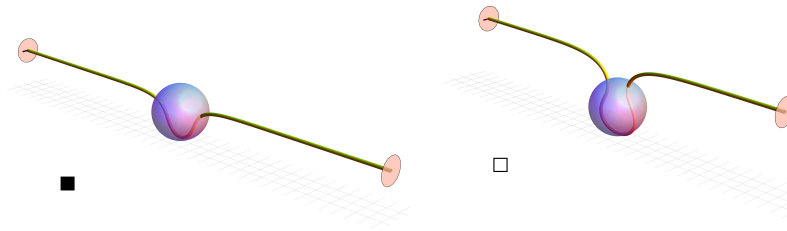
Fig. 6 2D configurations corresponding to the filled and empty squares on the post-buckling diagram of Figures 3 and 4.
