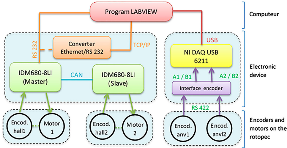
Figure 8. Automation structure of RoToPEc module.
