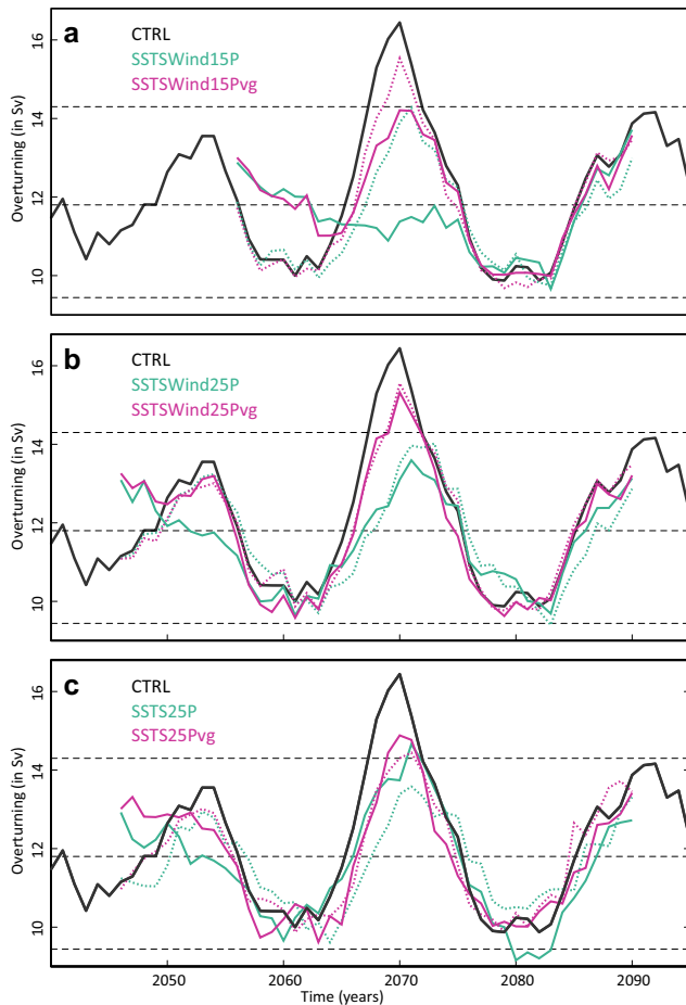
Fig. 9 Evolution of the MOI-48N-noek index in CTRL ( thick black line ) and both SSTSWind15P ( blue lines ) and SSTSWind15Pvg ( magenta lines ) experiments. Colored (dotted) lines account for experiments starting from moderate (exact) initial conditions. Horizontal grey dashed lines indicate the climatological mean and the 5th and 95th percentiles of the 1000-years CTRL. b, c Same as a but for the SSTS25P/SSTS25Pvg and SSTS25P/SSTS25Pvg experiments, respectively
