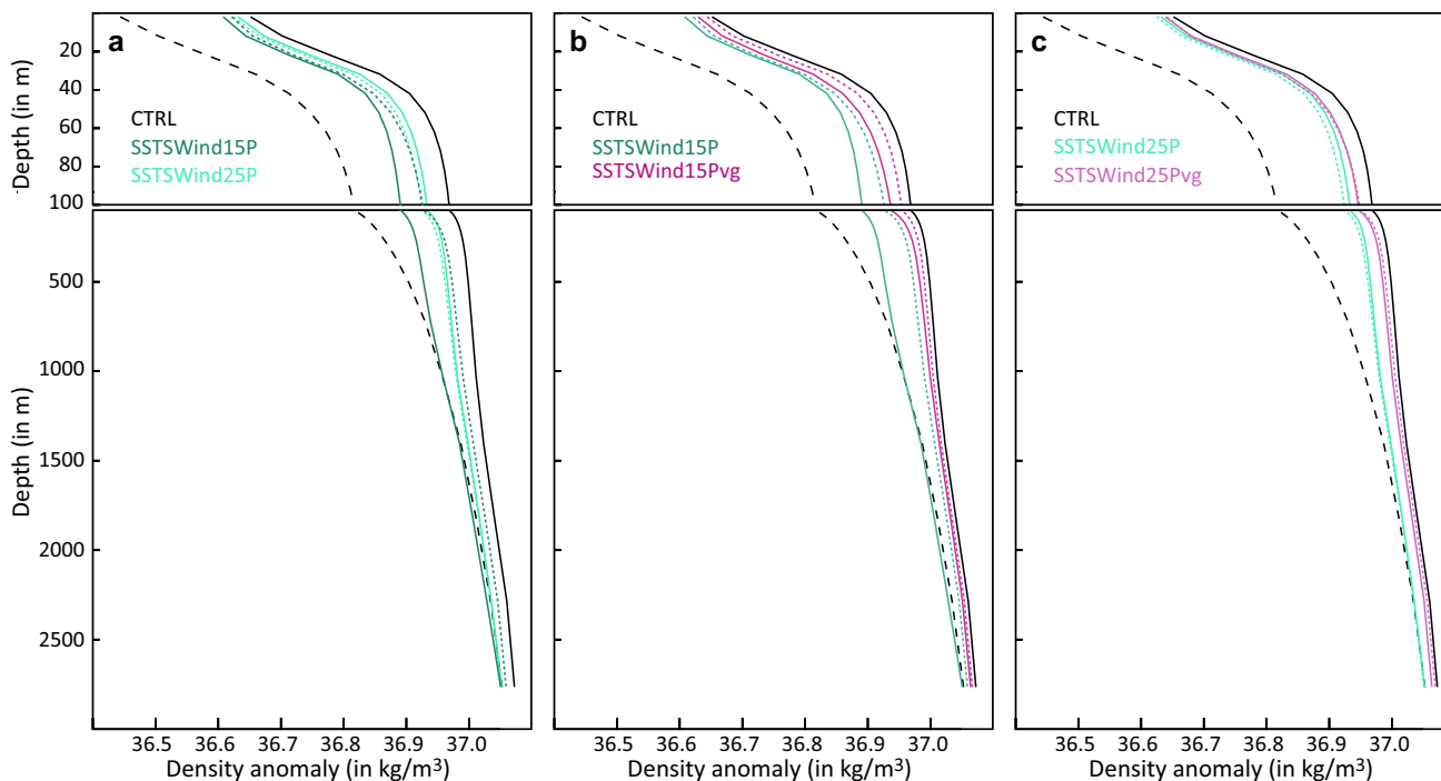
Fig. 8 Vertical profile of the mean density anomaly ( \sigma_2 ) in the southern convection region during the period 2063–2066 in CTRL and different sets of nudged experiments: a SSTSWind15P and SSTSWind25P, b SSTSWind15P and SSTSWind15Pvg, and c SSTSWind25P and SSTSWind25Pvg. Full (dotted) colored lines cor-
