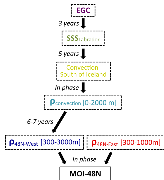
Fig. 1 Schematic of the AMOC precursors in the ISPL-CM5A-LR model, as identified in Escudier et al. (2013) and Ortega et al. (2015). The estimated leading times are indicated in the arrows
