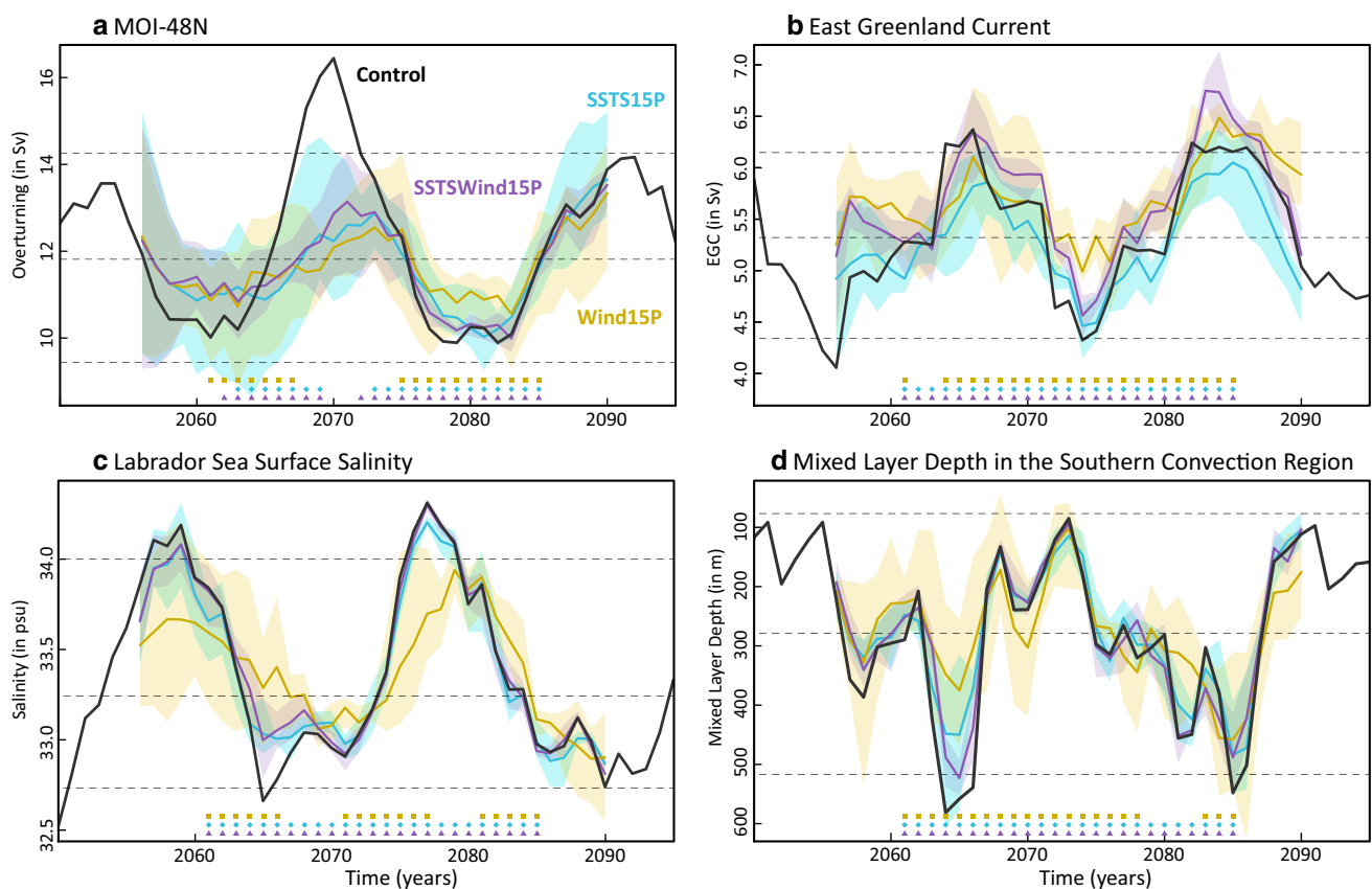
Fig. 4 a Evolution of the MOI-48N in CTRL and the nudged ensembles Wind15P, SSTS15P and SSTSWind15P. Colored envelopes represent the total ensemble spread, and thick colored lines the associated ensemble mean. Horizontal dashed lines mark the climatological mean and the associated 5th and 95th percentiles of the CTRL simulation. Symbols at the bottom of each panel highlight the centre of
