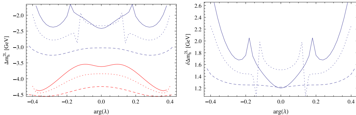
Fig. 12 On the left size of the two-loop corrections as function of \arg(\lambda) for different values of |\lambda| : 0.4 (dashed), 0.6 (dotted), 0.7 (full). The red lines include only corrections \mathcal{O}(\alpha_s\alpha_t) , while the blue lines
