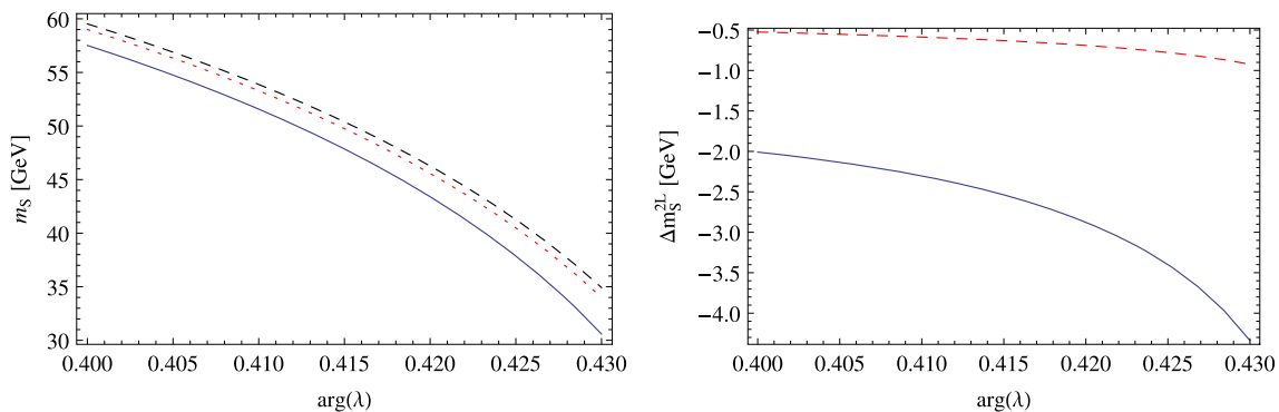
Fig. 13 On the left light singlet mass as a function of \arg(\lambda) for the benchmark scenario TP3 of Ref. [94]. The right side, show the size of the two-loop corrections \mathcal{O}(\alpha_s\alpha_t) only (dashed, red line), and of the
