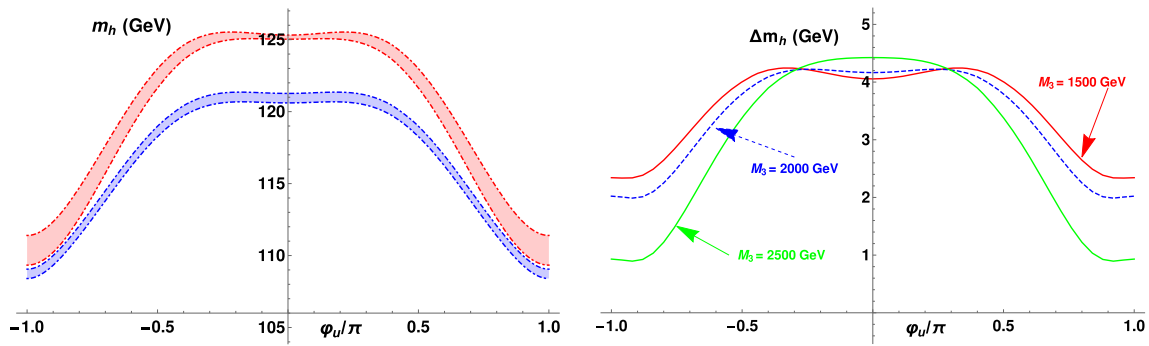
Fig. 9 Left plot of the lightest Higgs mass at one ( blue ) and two ( red ) loops as \varphi_U is varied. The bands show the variation between M_3 = 1500 GeV and 2500 GeV. Right difference between the one- and two-loop lightest Higgs masses for three different values of M_3 marked in the plot, as \varphi_U is varied
