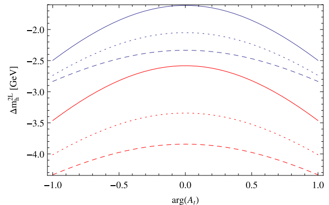
Fig. 11 Size of the two-loop corrections as a function of \arg(A_t) for different values of |A_t| : 1.5 TeV ( dashed ), 2.0 TeV ( dotted ), 2.5 TeV ( full ). The red lines include only corrections \mathcal{O}(\alpha_s \alpha_t) , while the blue lines include all other corrections in the gaugeless limit approximation
