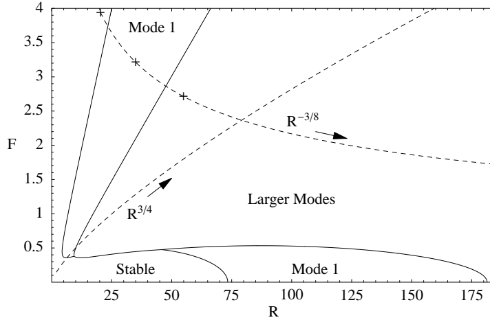
FIG. 5: Stability diagram for a laminar channel. The domains (separated by solid lines) are named after the most instable mode between n = 1 and n = 2 . The parameters values are \beta = 3.75 , \gamma = 1 and S = 0.0875 . The dashed lines represent the evolution of a straight river when the water level is imposed ( F = F_0(R/R_0)^{3/4} ) or when the outflow is imposed ( F = F_0(R/R_0)^{-3/8} ). The three cross correspond to the three cases presented in figure 4.
