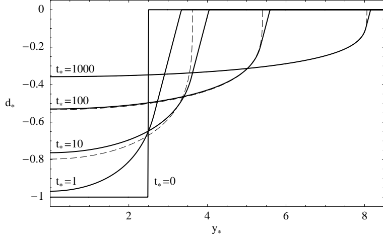
FIG. 3: Widening of a straight laminar channel through erosion, modelled with (16). Parameter values are \epsilon_a = 0.1 , \alpha = 0.8 , and \beta = 3.75 . Solid lines: numerical solutions of (16) at different times. Dashed line: self-similar solution (without avalanches, see section III B) at t_* = 10 , t_* = 100 and t_* = 1000 . The presence of avalanches seems not to influence much the self-similar evolution of the profile.
