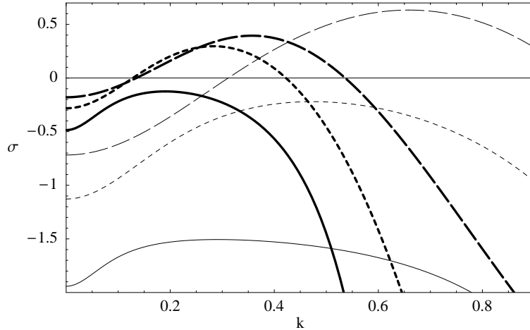
FIG. 4: Linear growth rate \sigma of bed instability in a laminar river, versus the corresponding non-dimensional wave number k . The fixed parameters values are \beta = 3.75 , \gamma = 1 , S = 0.0875 . The Froude number and aspect ratio are varied according to a straight river widening (see section IV B and figure 5). Solid curves : R = 20.3 and F = 3.94 . Short dashes : R = 35.0 and F = 3.21 . Long dashes : R = 55.0 and F = 2.71 . For each set (R, F) , the thick curve corresponds to the mode n = 1 , whereas the thin one correspond to the mode n = 2 . This behaviour provides an interpretation for the transition in patterns observed experimentally by [12].
